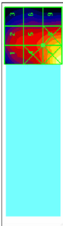
Figure 9-2 Sample H-field Scan Overlay (See Test Setup Photographs for actual WD overlay)
