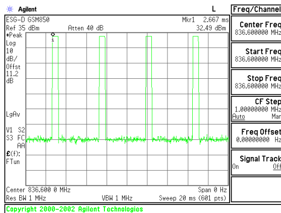
Figure 8-4 GSM850 Signal
