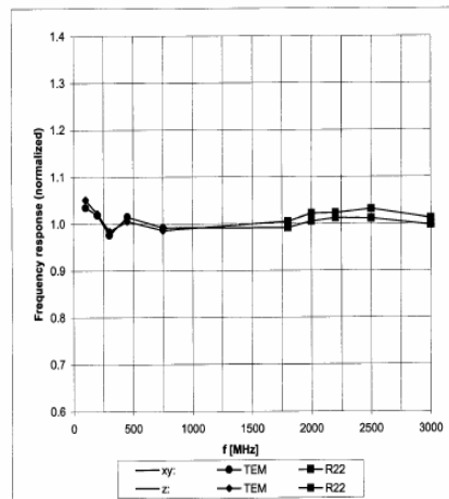
Frequency Response of H-Field (TEM-Cell: if1110, Waveguide R22)
