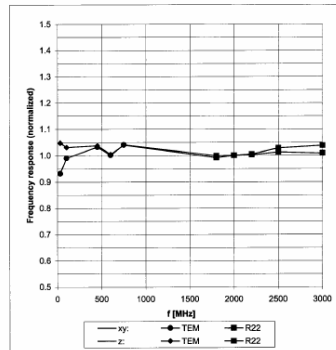
Frequency Response of E-Field (TEM-Cell: if1110 EXX, Waveguide R22)
