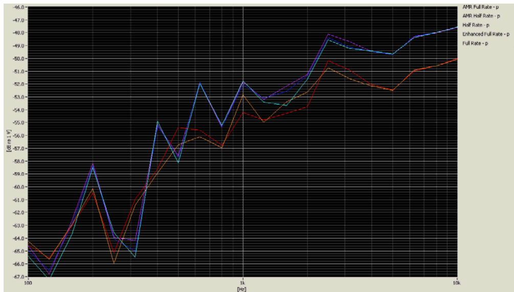
Figure 5-8 Vocoder Analysis for ABM Noise
