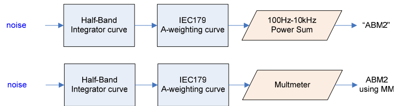
Figure 5-6 ABM2 Validation Block Diagram
