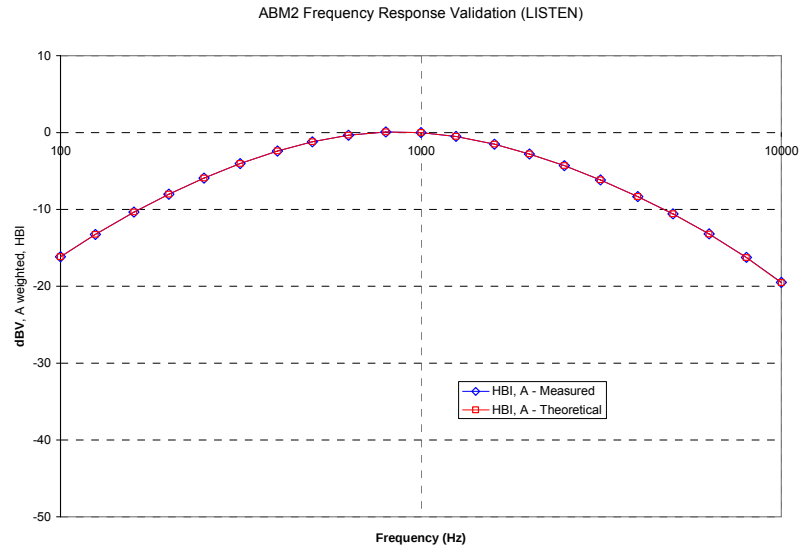
Figure 5-5 ABM2 Frequency Response Validation
