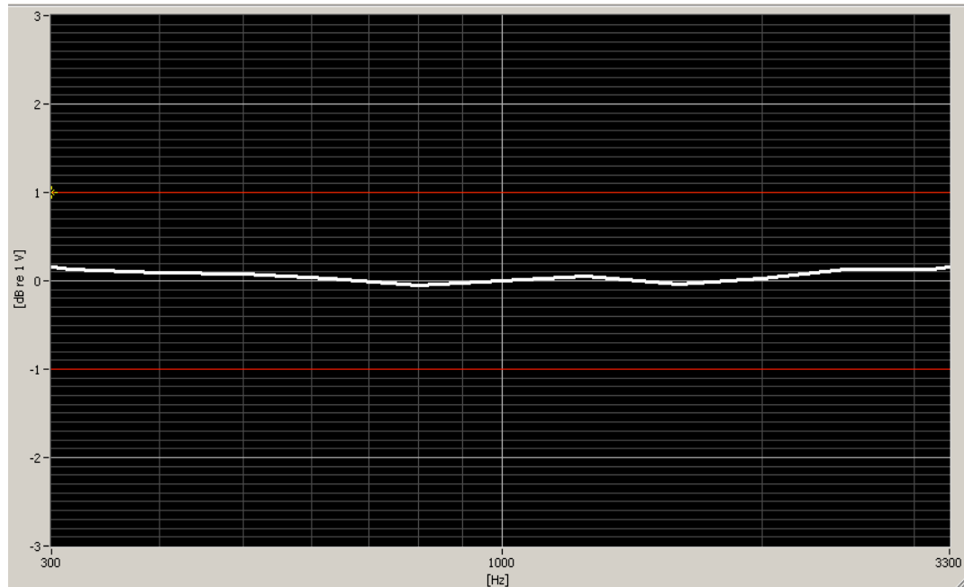
Figure 6-2 Helmholtz Coil Validation for Frequency Response
