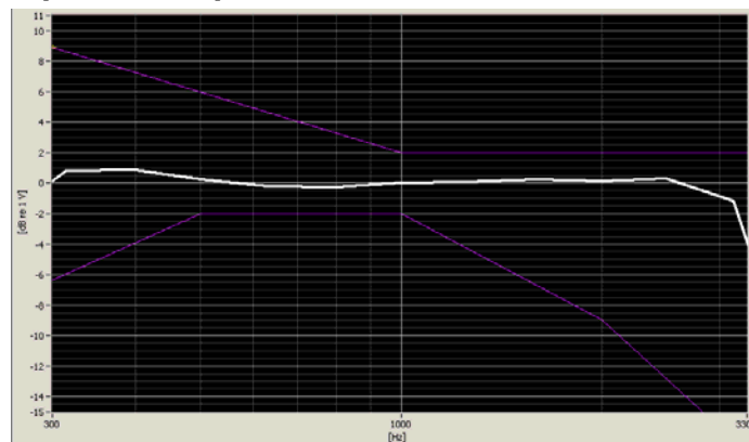
Figure 6-1 Axial Frequency Response
