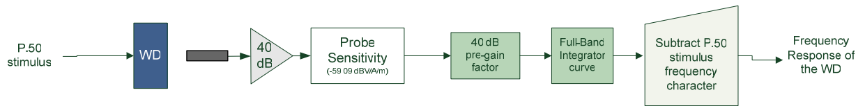
Figure 5-9 Frequency Response Block Diagram
