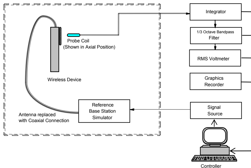
Figure 5-10 Audio Magnetic Field Test Setup
