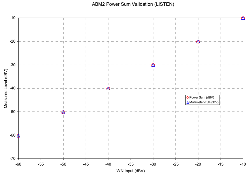
Figure 5-7 ABM2 Power Sum Validation
