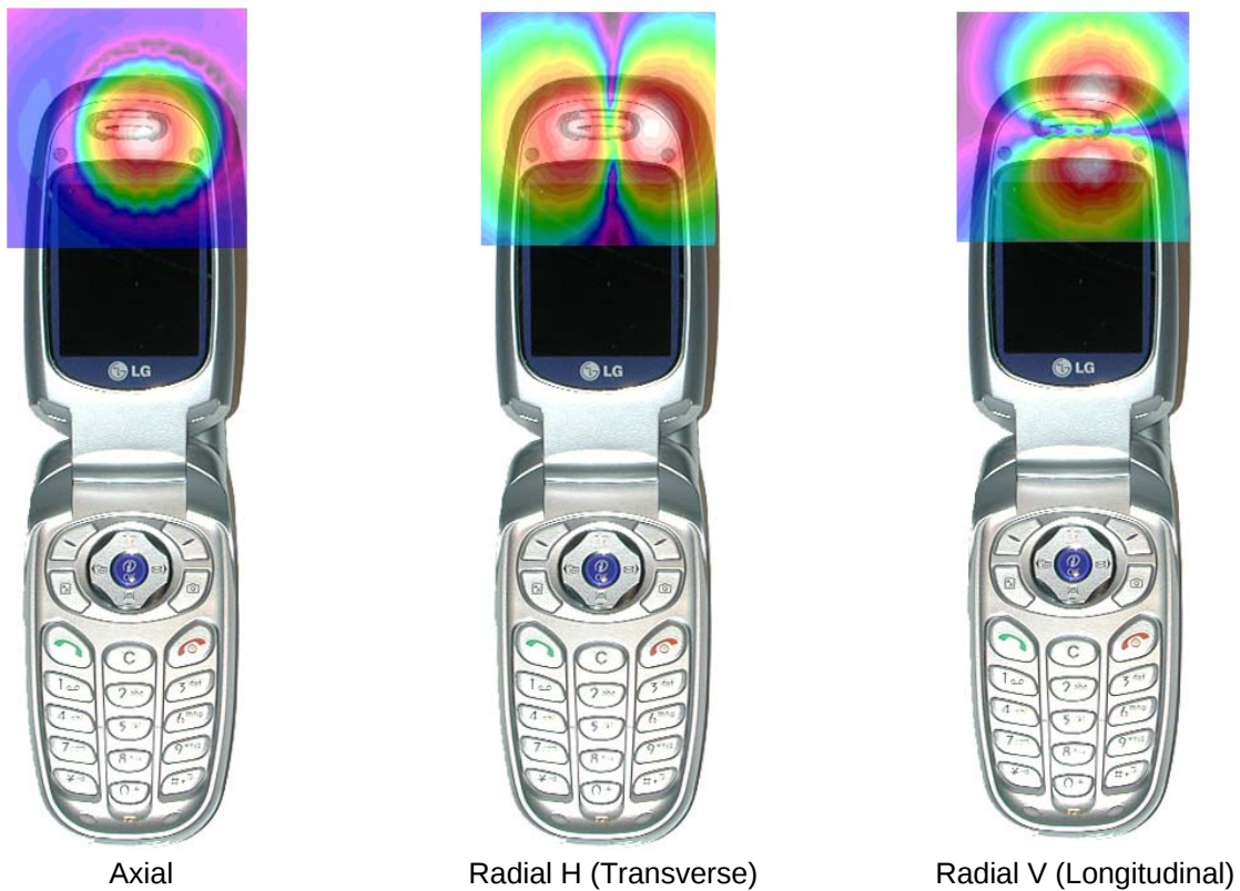
Figure 12-3 T-Coil Scan Overlay Magnetic Field Distributions
