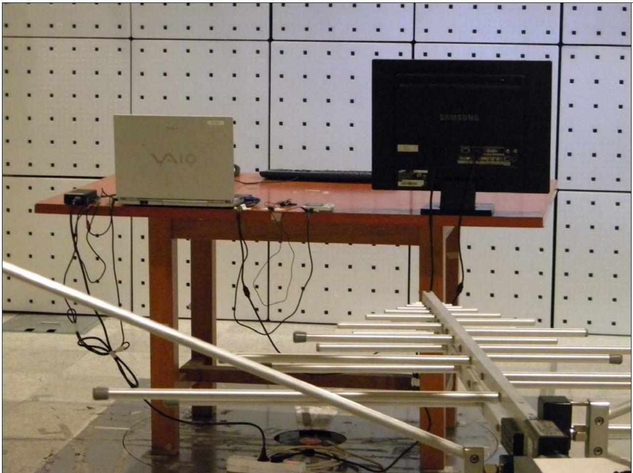
RE Rear
