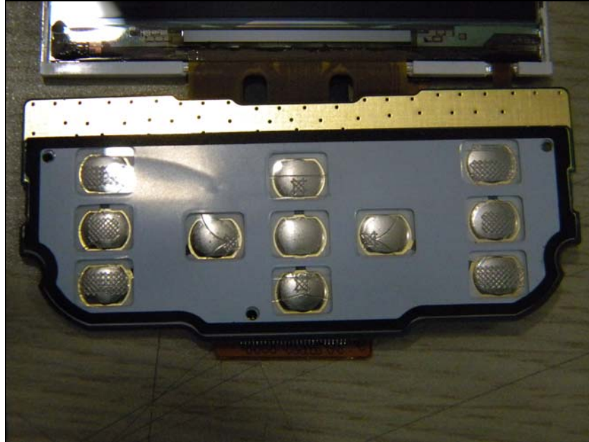
Key pad Front
