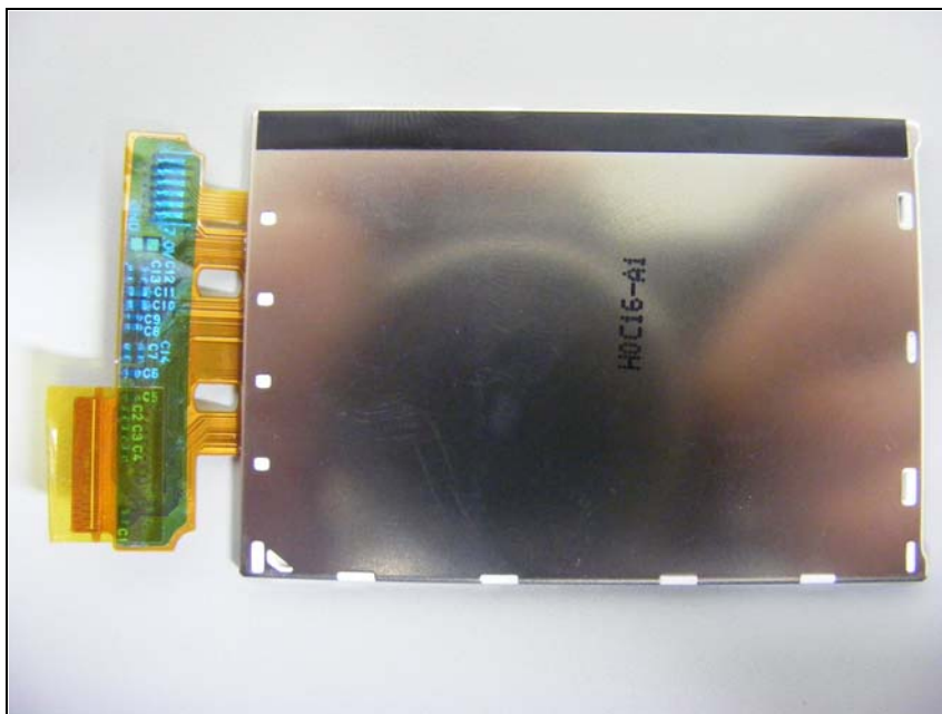
Bottom view of LCD module
