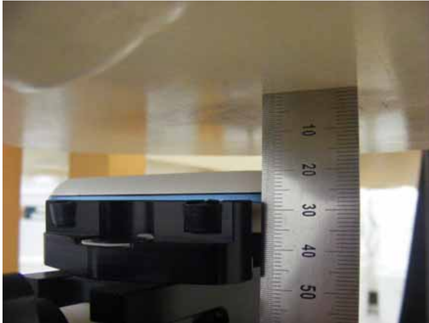
Body Front_Slide Down
