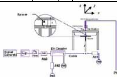
Figure 9.1 Dipole Validation Test Setup
