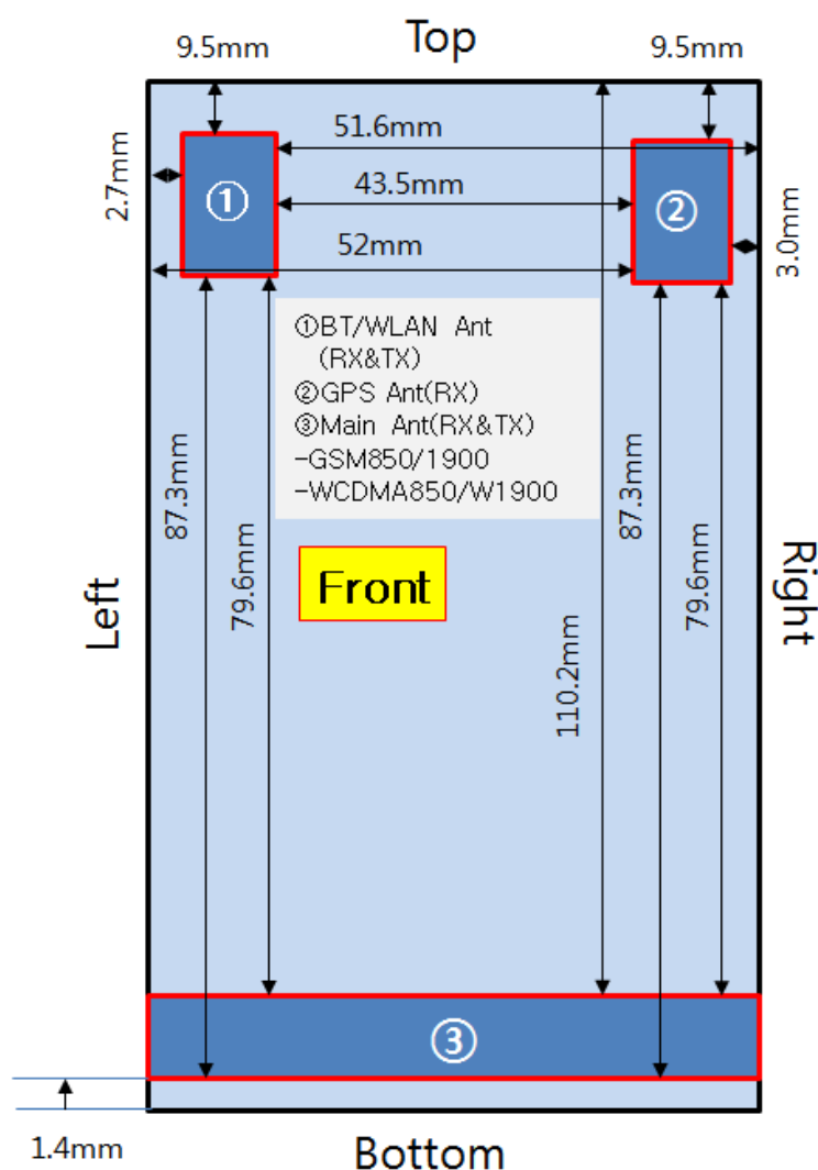
Figure 13.1 Identification of Sides for SAR Testing
