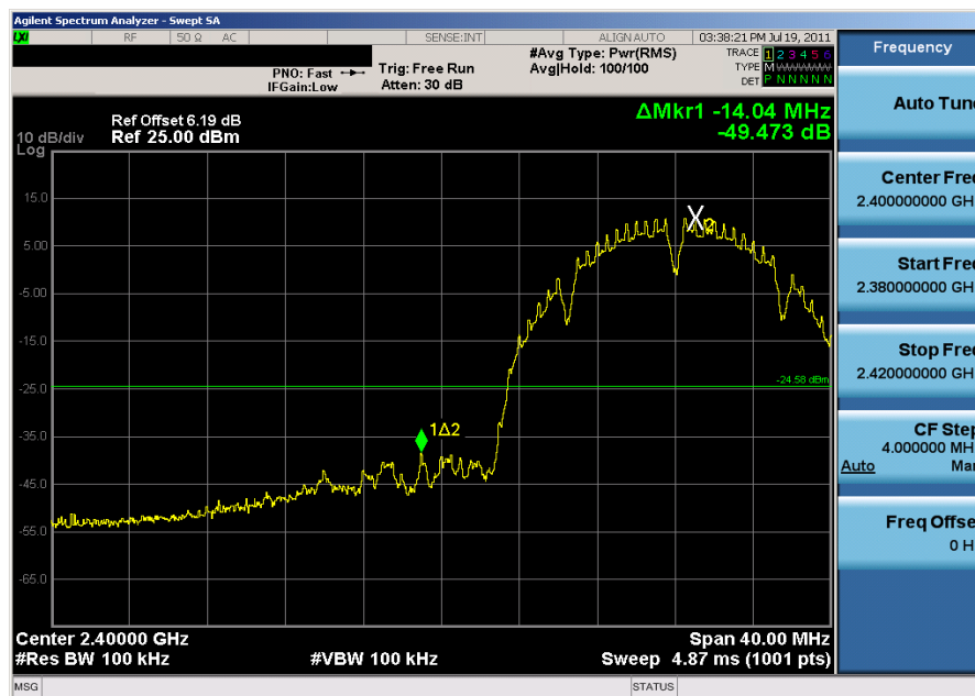
Plot 6-19. Band Edge Plot (802.11b – Ch. 1)
