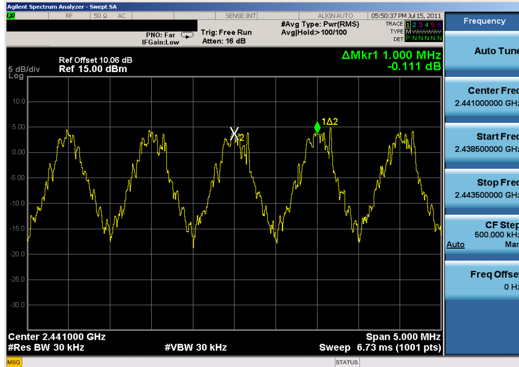
Plot 6-14. Channel Spacing Plot (Bluetooth)
