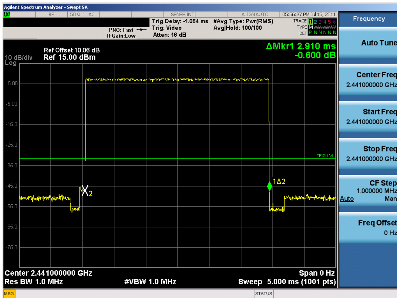
Plot 6-15. Time of Occupancy Plot (Bluetooth)
