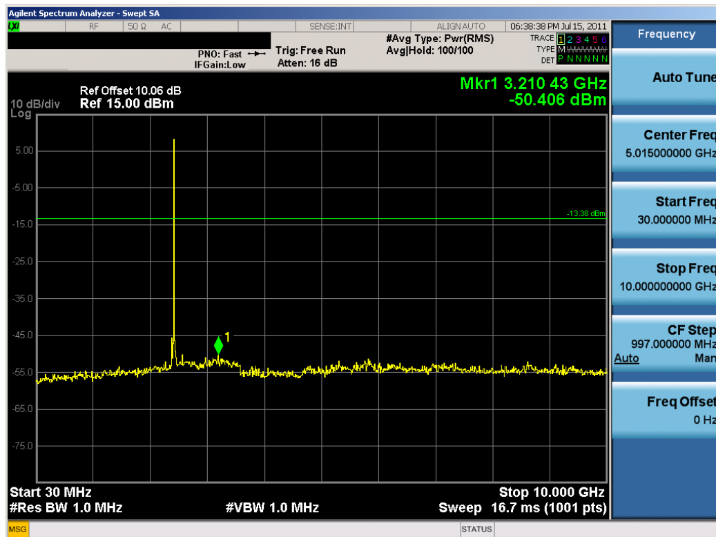
Plot 6-20. Conducted Spurious Plot (Bluetooth, 2Mbps – Ch. 39)
