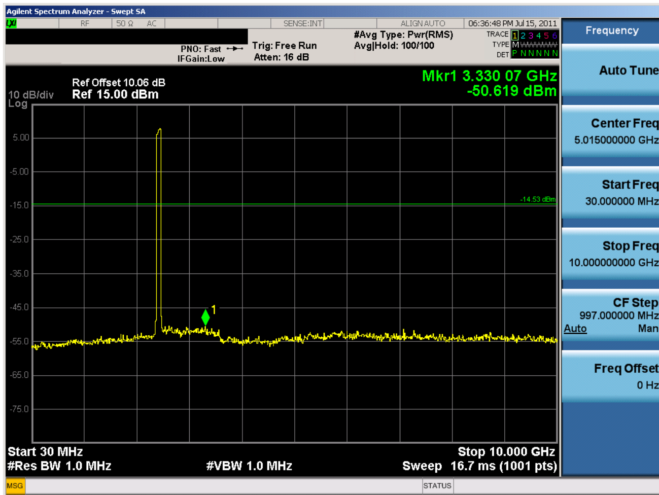
Plot 6-18. Conducted Spurious Plot (Bluetooth, 2Mbps – Ch. 0)
