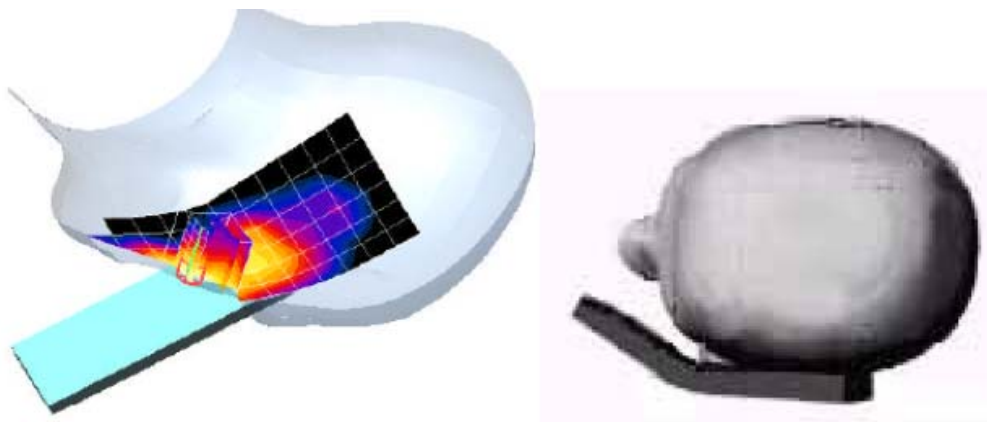
Figure 7.4 SAR Scans near the Jaw / Mouth
