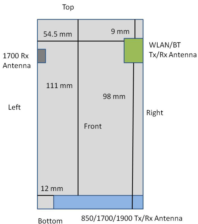
Figure 13-1 Identification of Sides for SAR Testing
