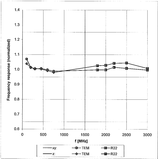
Uncertainty of Frequency Response of H-field: \pm 6.3\% ( k=2 )
