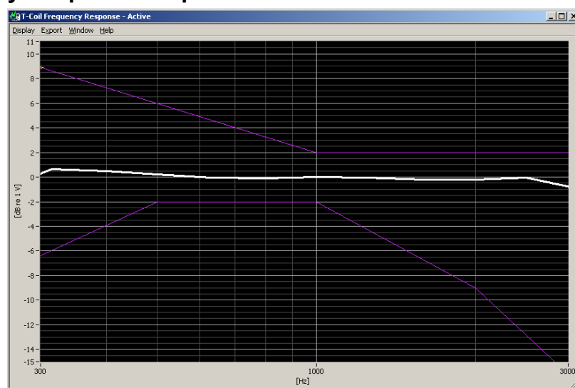
Figure 7-1 Axial Frequency Response
