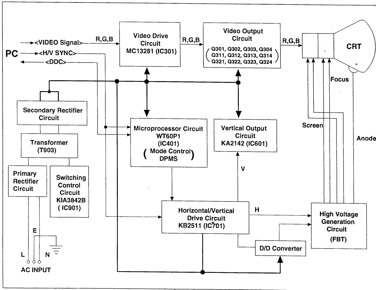
BLOCK DIAGRAM
