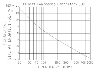
Fig. 5. NSA Theoretical Attenuation Curves (Horiz. Pol.)
