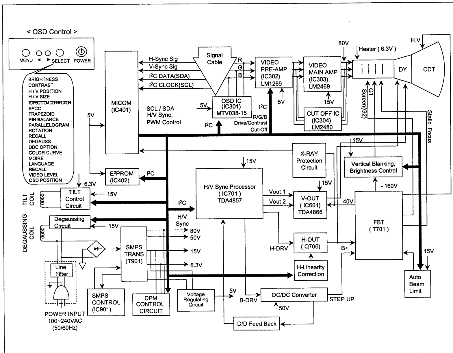
BLOCK DIAGRAM
