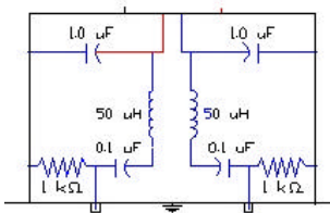
Fig. 3. LISN Schematic Diagram
