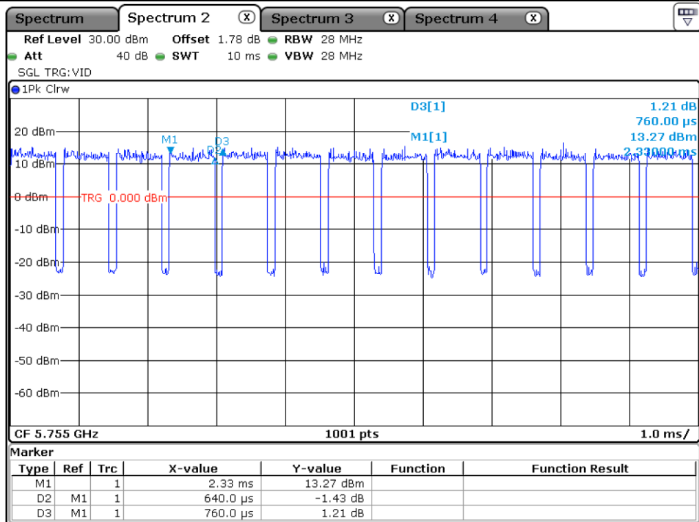
UNII 3_802.11ac(VHT40)_Antenna 0
