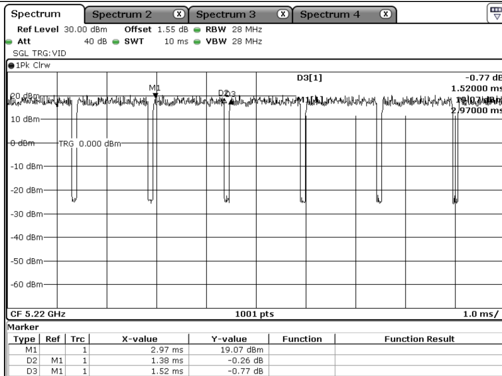
UNII 1_802.11a_Antenna 0
