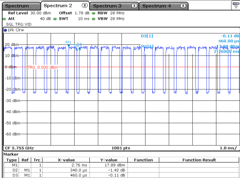
UNII 3_802.11ac(VHT20)_Antenna 0
