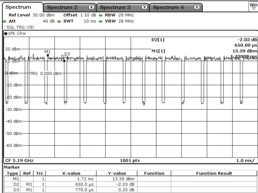
UNII 1_802.11ac(VHT40)_Antenna 0
