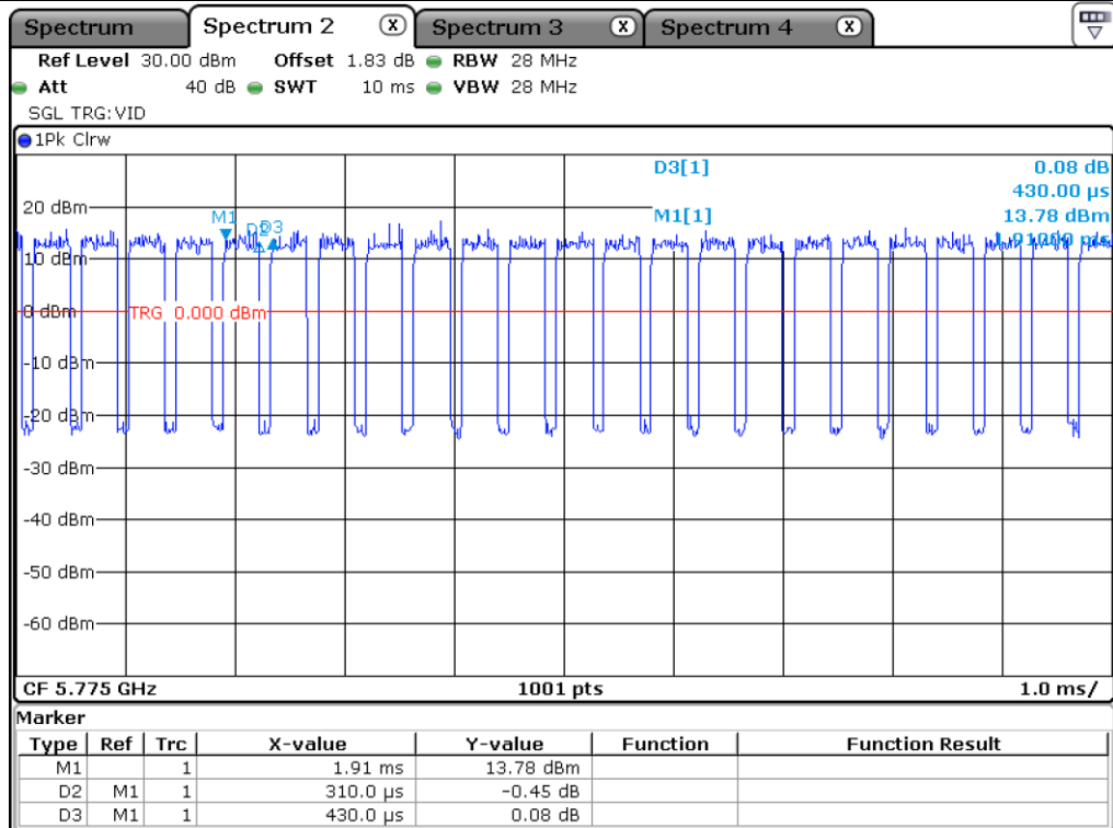
UNII 3_802.11ac(VHT40)_Antenna 1
