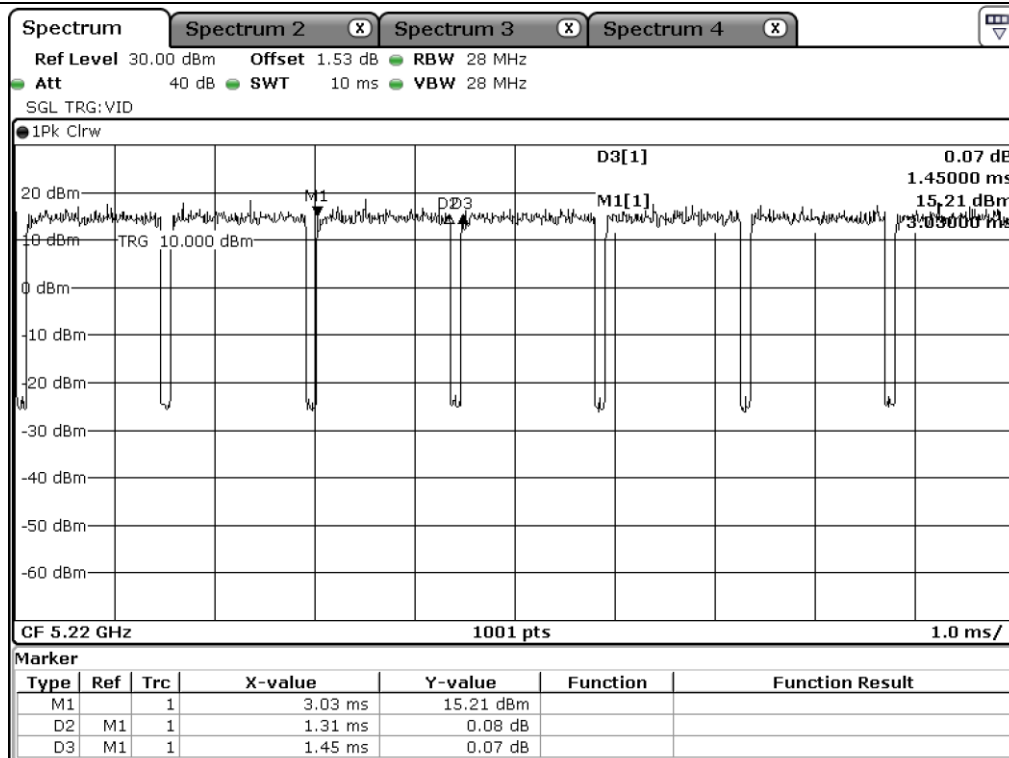
UNII 1_802.11ac(VHT20)_Antenna 1
