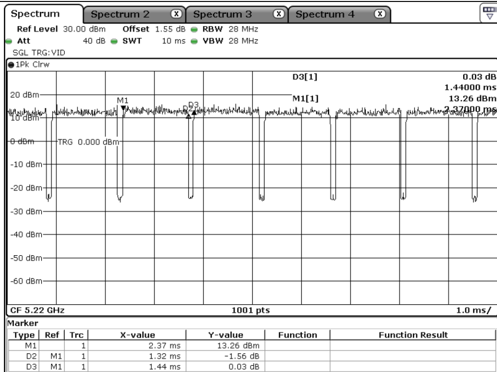
UNII 1_802.11ac(VHT20)_Antenna 0
