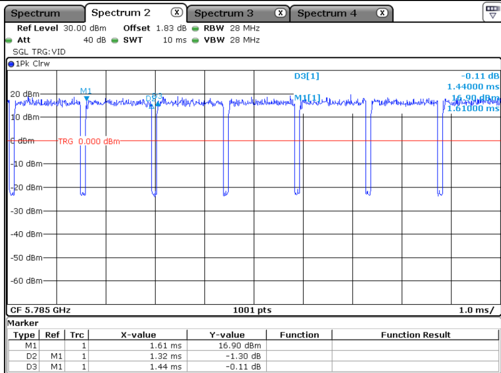
UNII 3_802.11ac(VHT20)_Antenna 1
