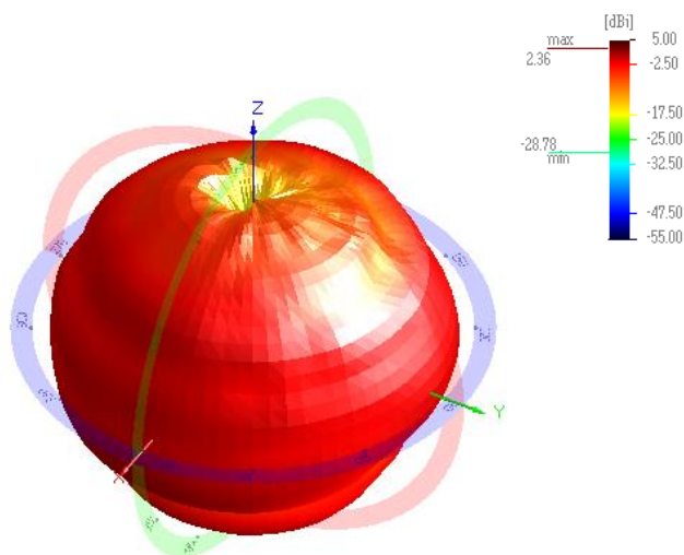
[3D Radiation Pattern @2450MHz]
