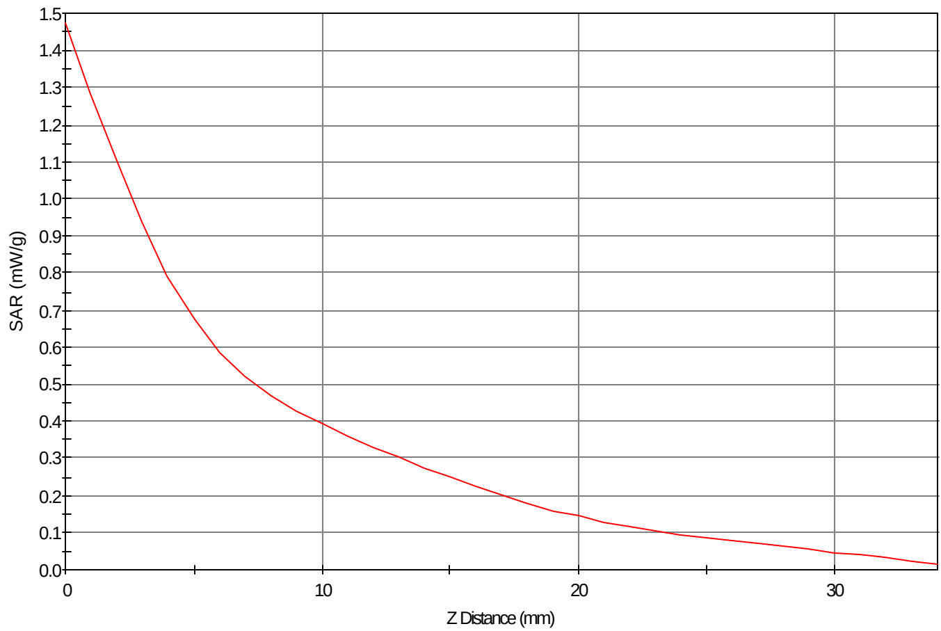
SAR - Z Axis at Hotspot x:-15.0 y:37.0
