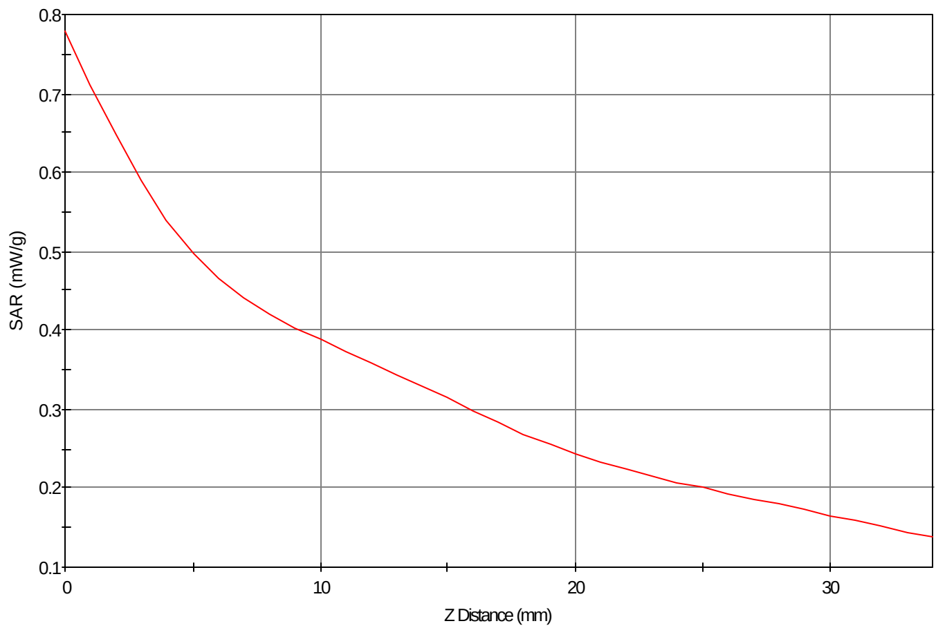
SAR - Z Axis at Hotspot x:68.0 y:9.0
