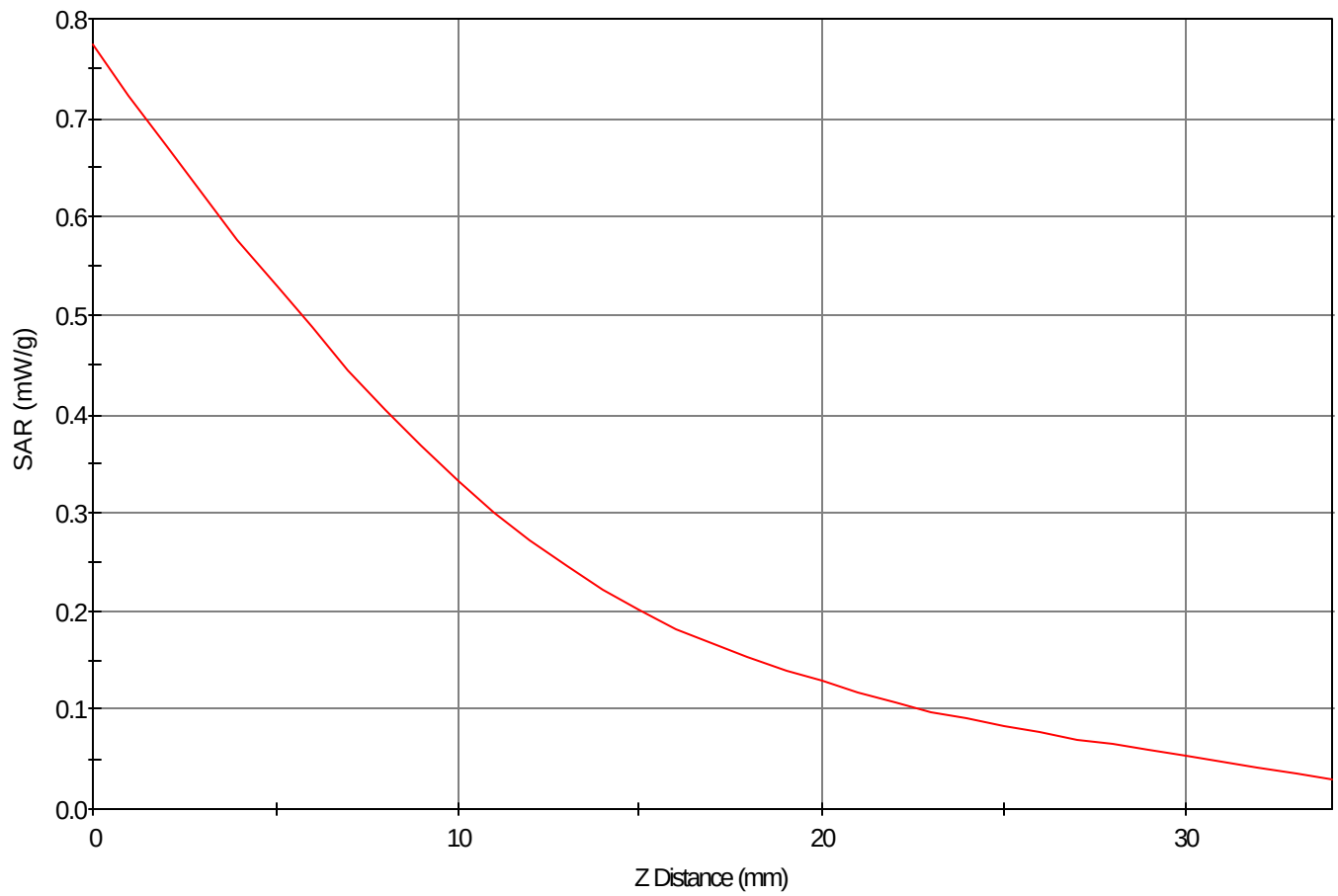
SAR - Z Axis at Hotspot x:68.0 y:3.0
