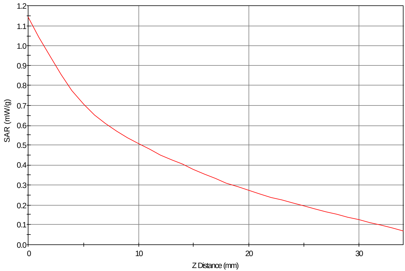
SAR - Z Axis at Hotspot x:36.0 y:6.0
