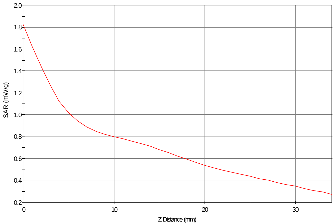
SAR - Z Axis at Hotspot x:-13.0 y:35.0
