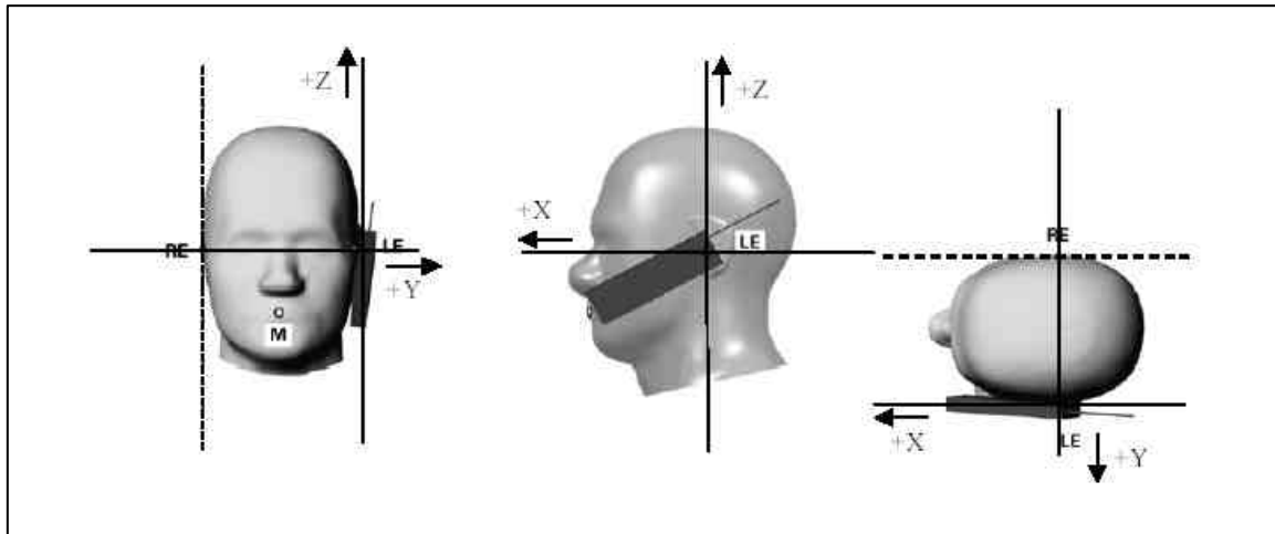
Figure 12.1 Handset Reference Points
