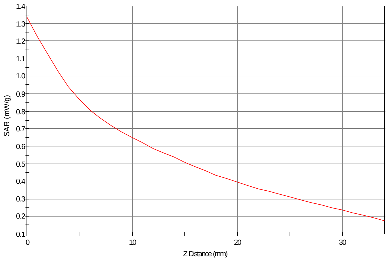
SAR - Z Axis at Hotspot x:80.0 y:19.0
