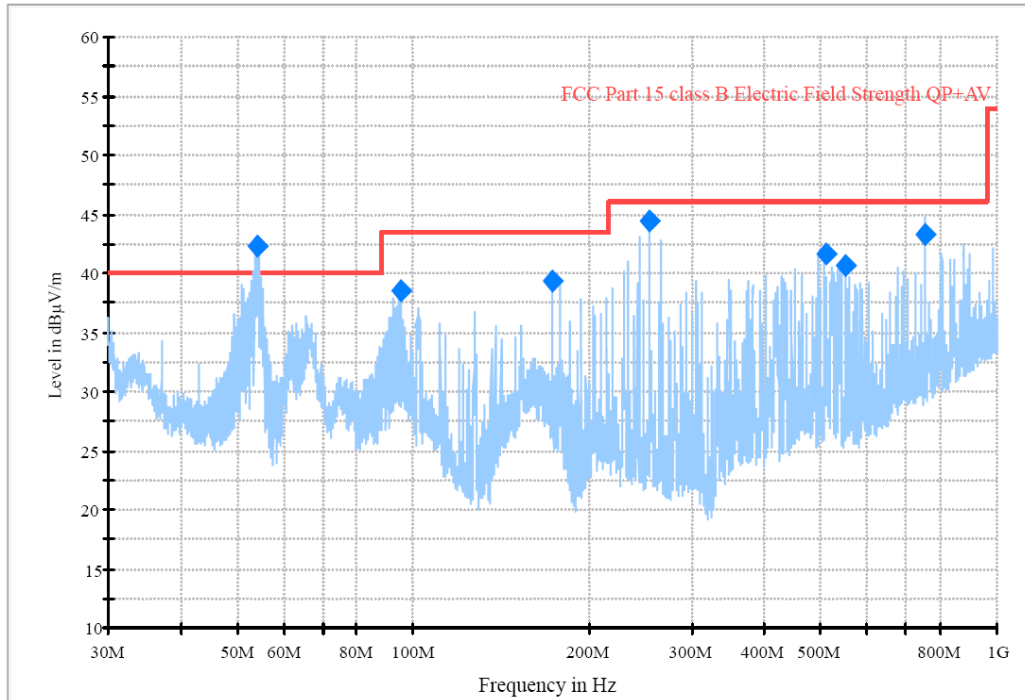
ESCI_Radiated Field Strength_30M_1GHz
