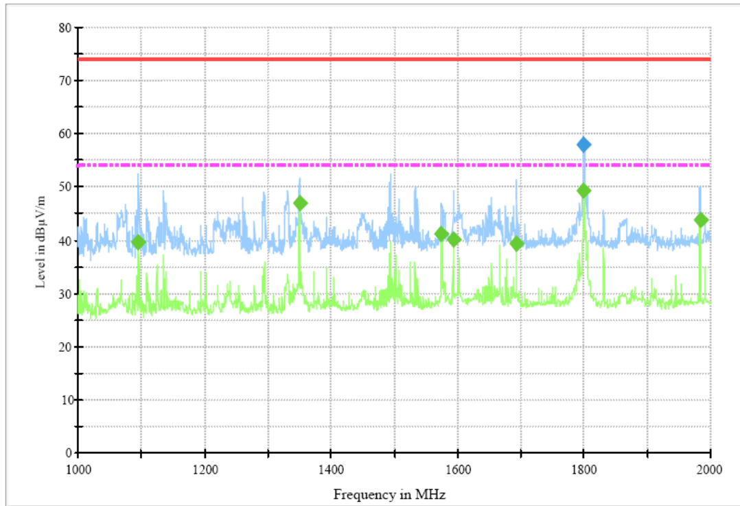
FCC_ESIB_Preamplifier_RE with Scans
