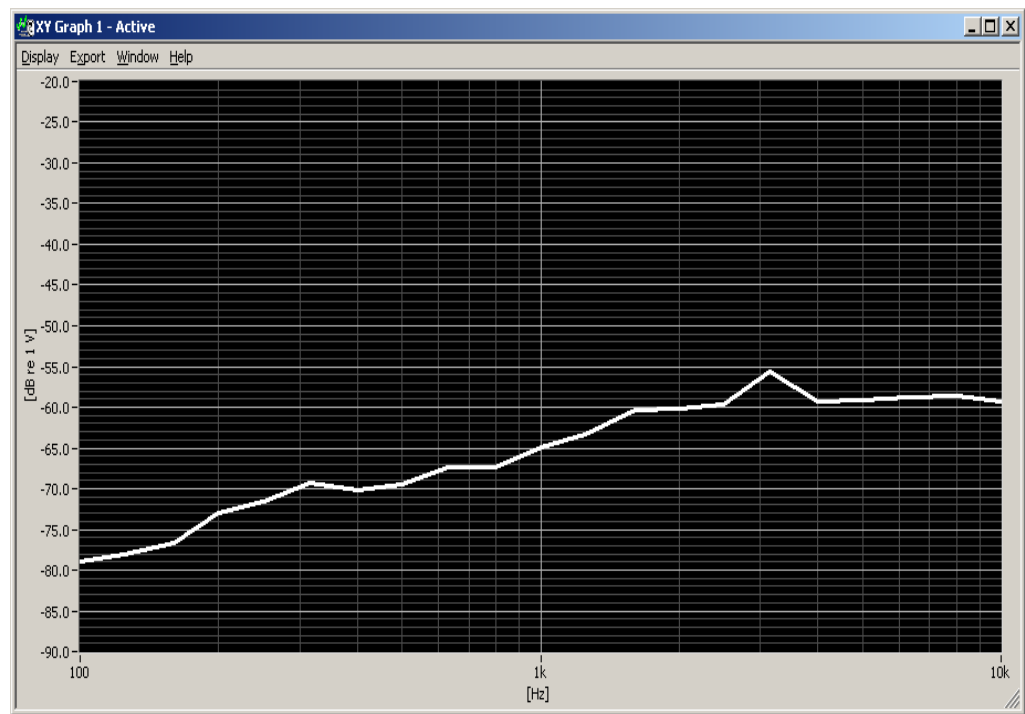
Figure 7-2 Worst-case ABM2 Plot for WD
