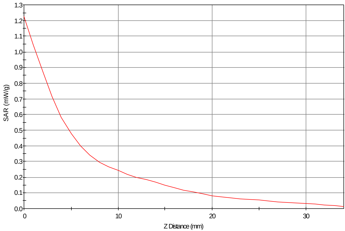
SAR - Z Axis at Hotspot x:-4.0 y:-15.0
