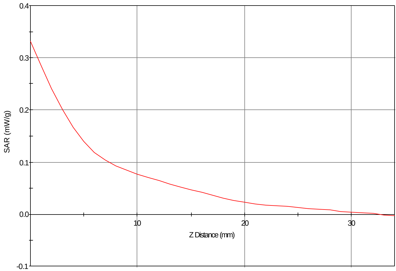
SAR - Z Axis at Hotspot x:66.0 y:-2.0
