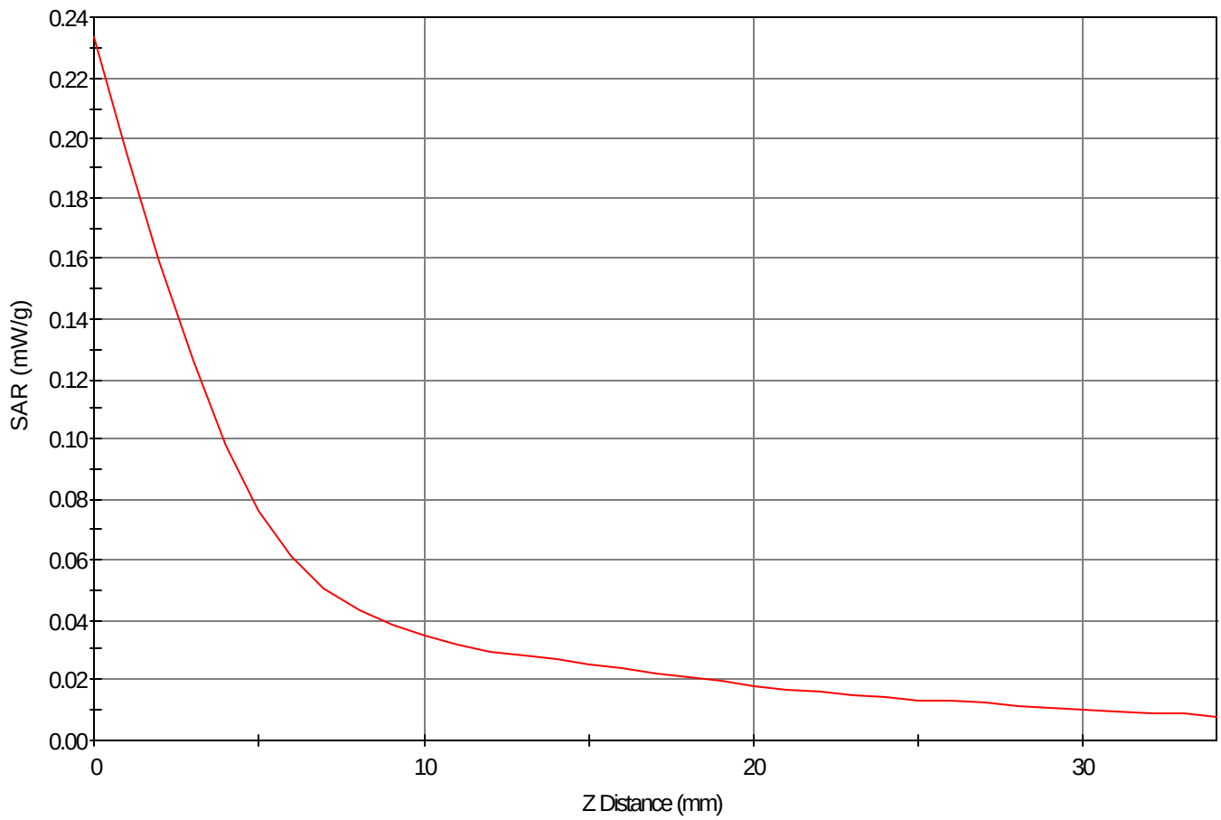
SAR - Z Axis at Hotspot x:22.0 y:6.0
