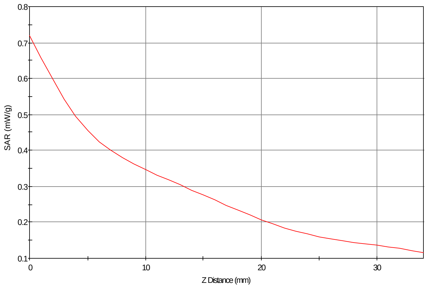
SAR - Z Axis at Hotspot x:73.0 y:3.0
