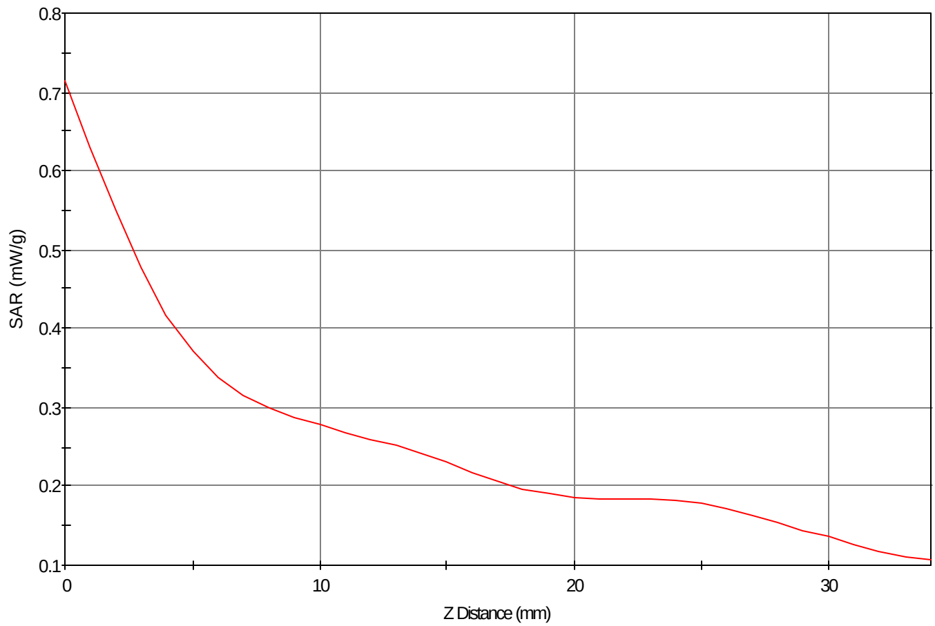
SAR - Z Axis at Hotspot x:52.0 y:3.0
