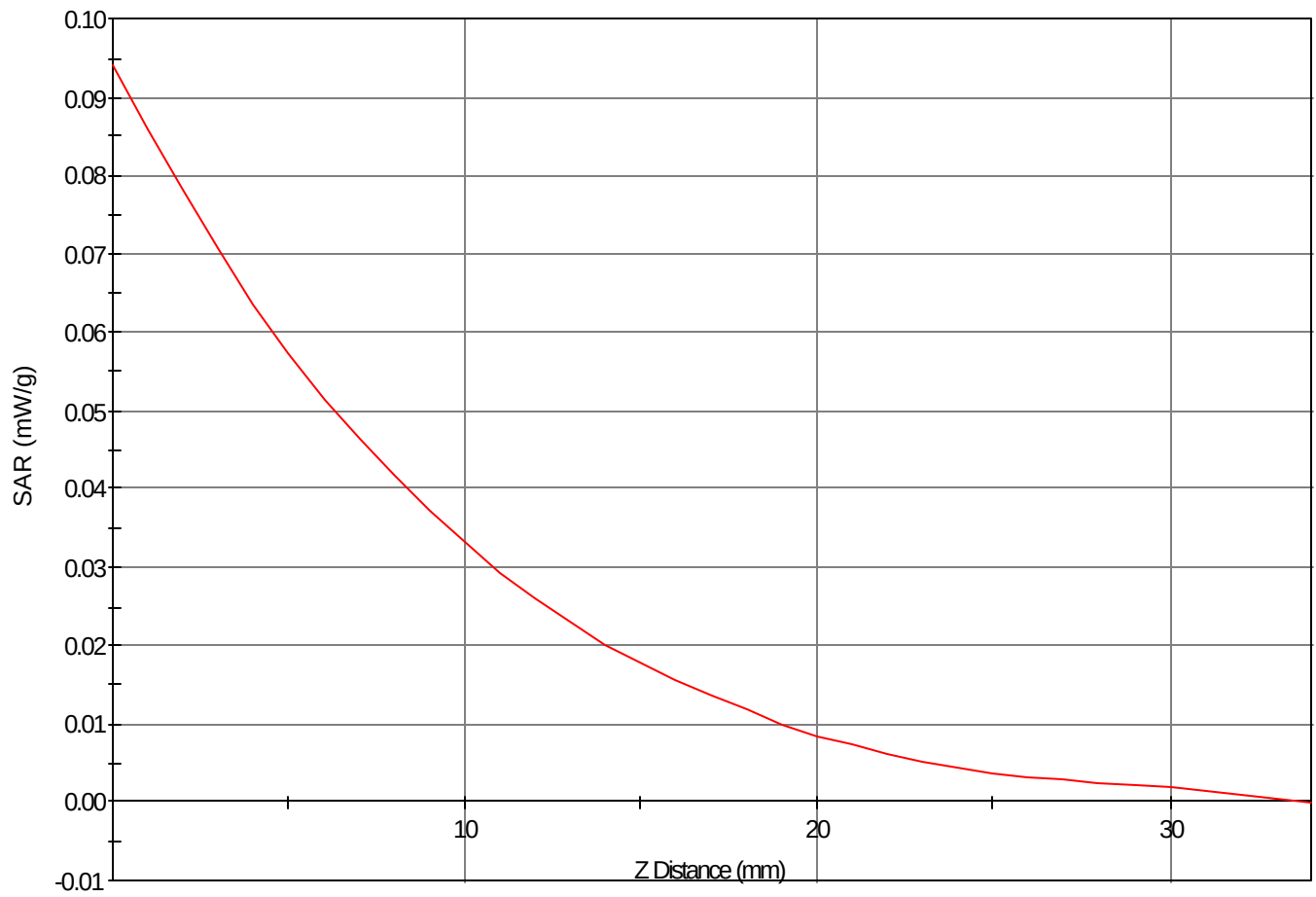
SAR - Z Axis at Hotspot x:72.0 y:2.0
