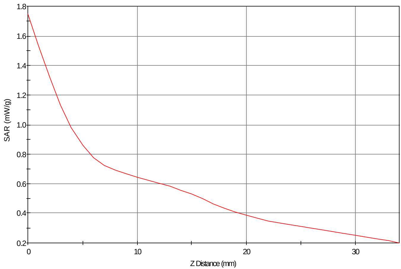
SAR - Z Axis at Hotspot x:72.0 y:5.0
