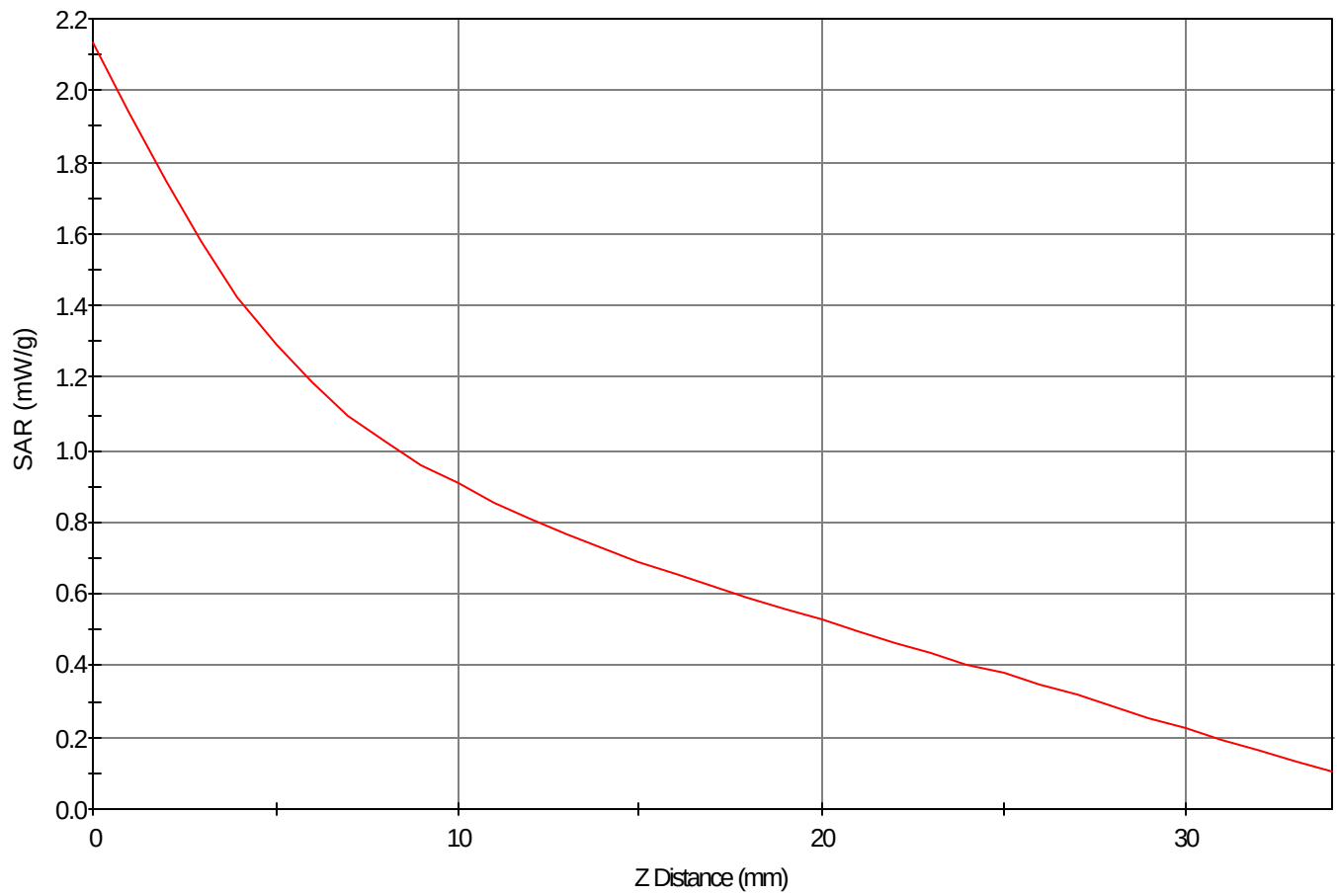
SAR - Z Axis at Hotspot x:-3.0 y:-7.0
