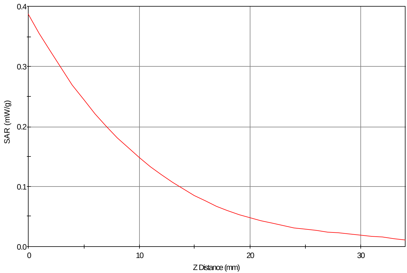
SAR - Z Axis at Hotspot x:67.0 y:2.0
