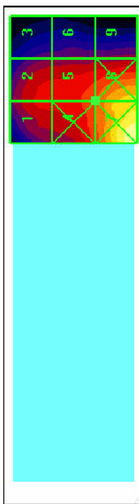
Figure 9-2 Sample H-field Scan Overlay (See Test Setup Photographs for actual WD overlay)
