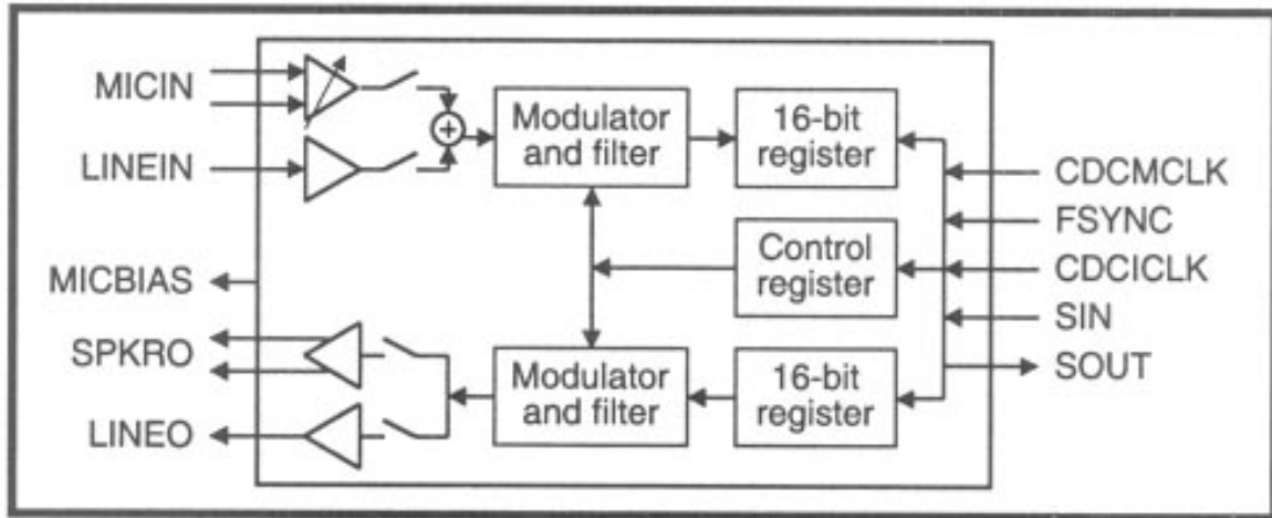
CKTU-24 CODEC Block Diagram
