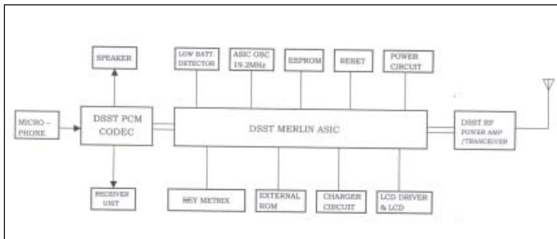
CKTU-24 Hand Block Diagram
