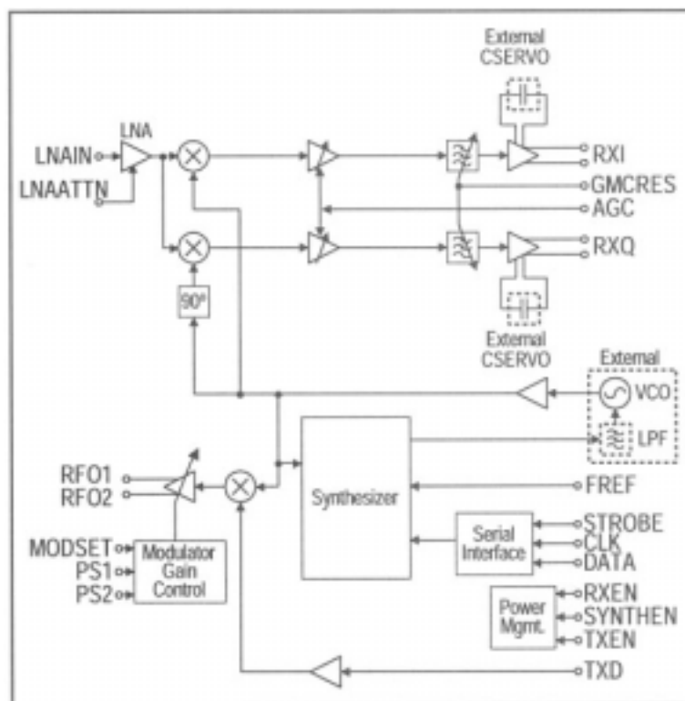
CKTU-24 RF Block Diagram
