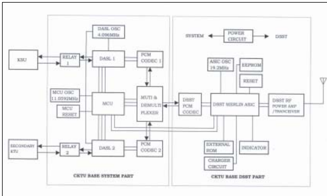
CKTU-24 Base Block Diagram
