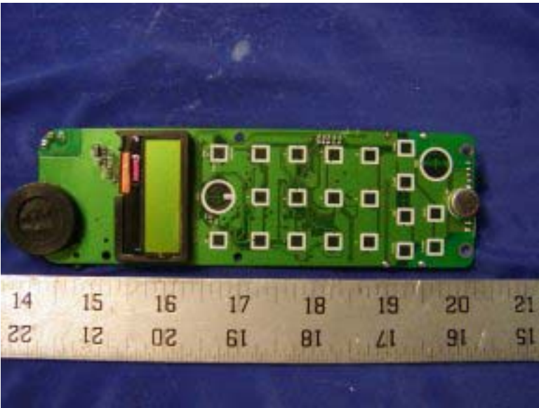
Handset - Main Board Solder View
