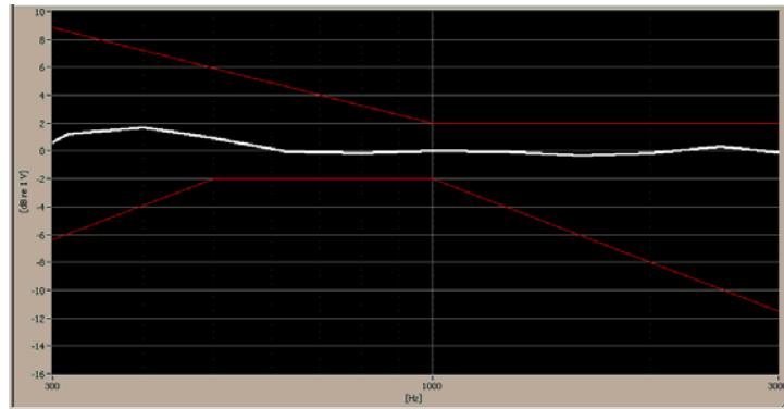
Figure 6-1 Axial Frequency Response
