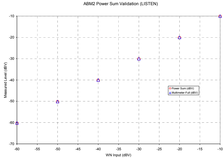
Figure 5-10 ABM2 Power Sum Validation
