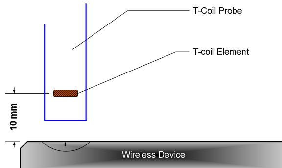
Figure 5-11 Measurement Distance
