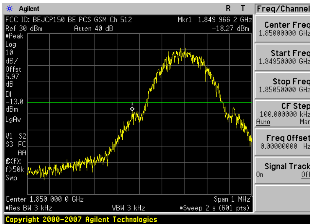
Plot 7-12. Band Edge Plot (PCS GSM Mode – Ch. 512)
