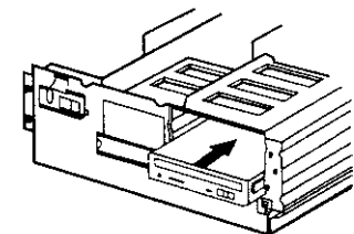
Figure 7. Mounting the Drive
