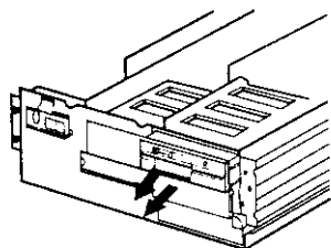
Figure 6. Removing the Floppy Disk Drive and the Blanking plate
