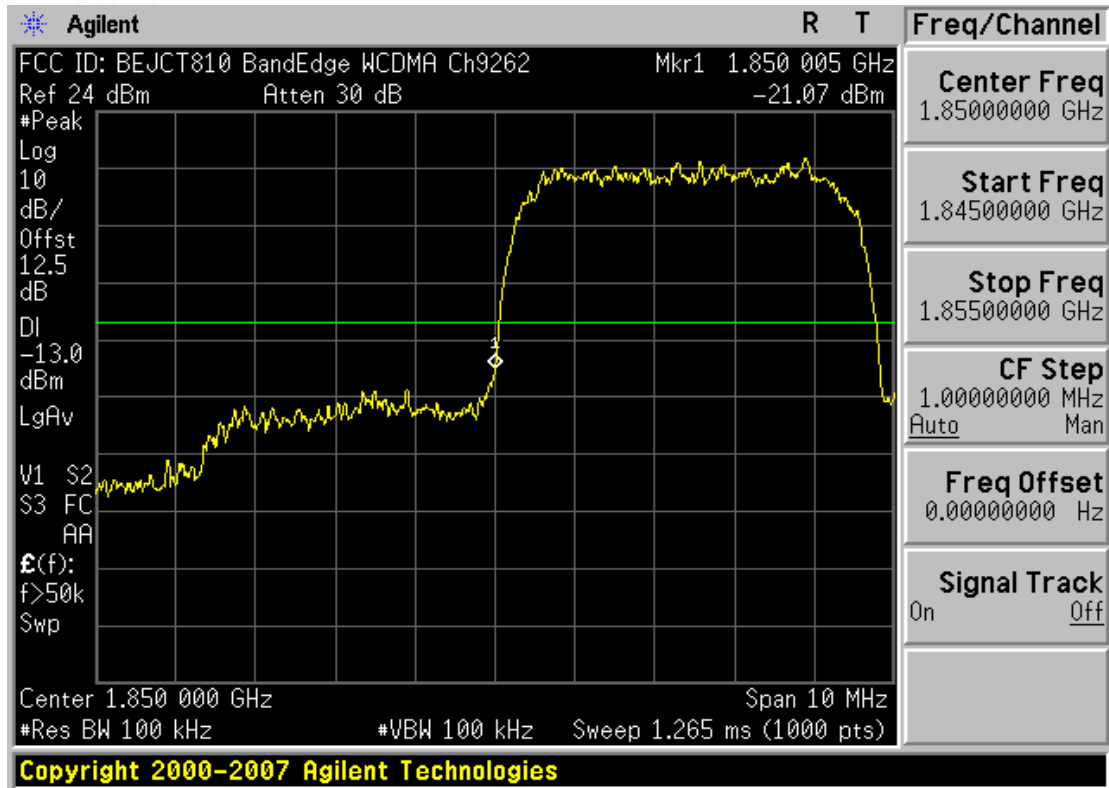
Plot 7-35. Band Edge Plot (PCS WCDMA Mode – Ch. 9262)
