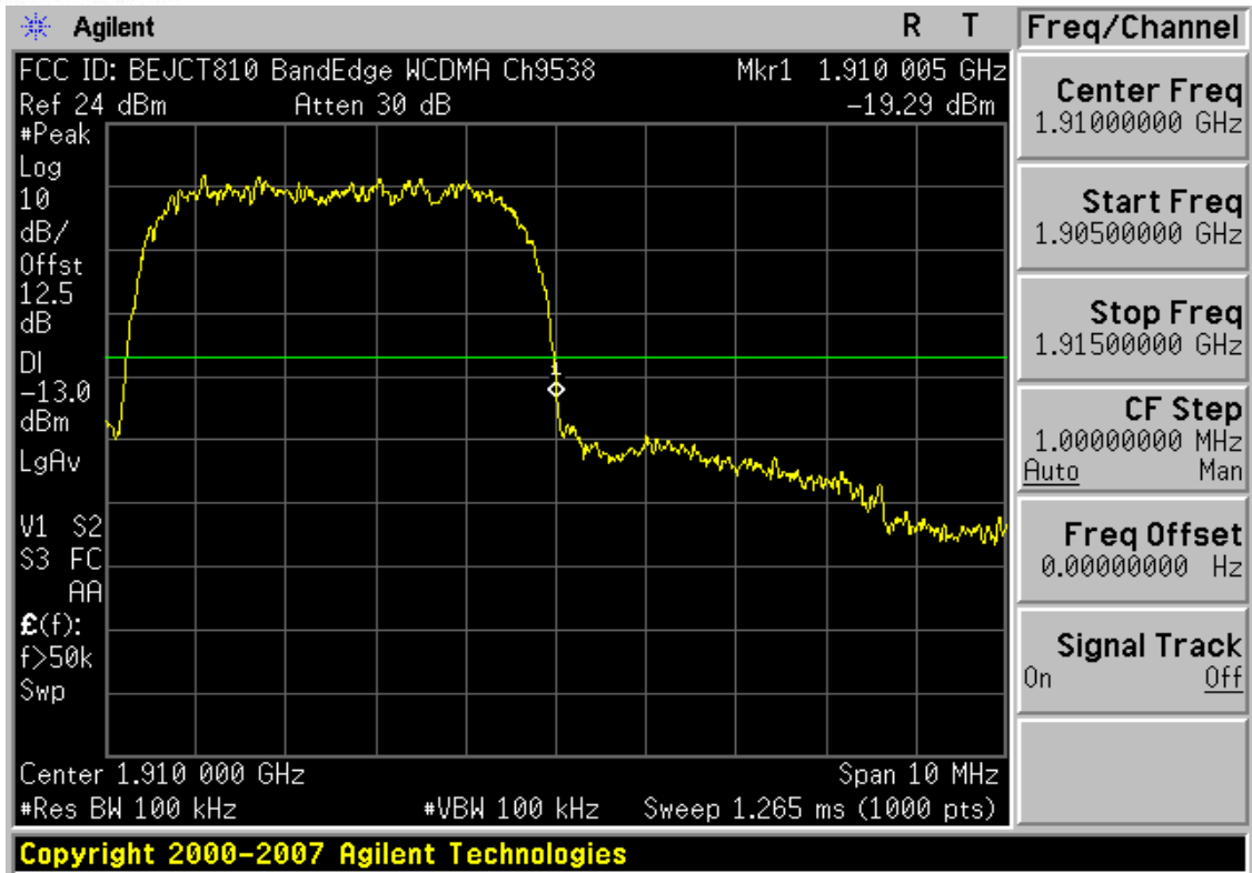
Plot 7-43. Band Edge Plot (PCS WCDMA Mode – Ch. 9538)
