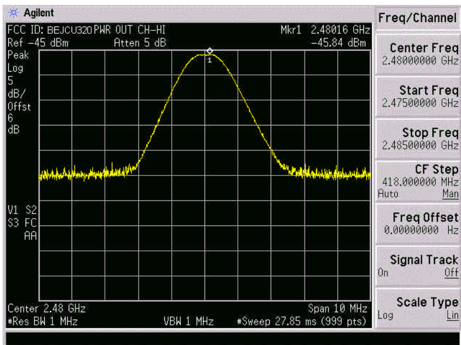
Plot A-6. Max. Peak Output Power Plot – Ch. 89
