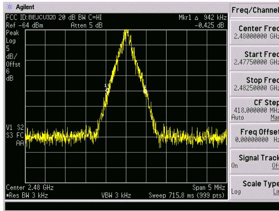
Plot A-3. 20dB Bandwidth Plot – Ch. 79
