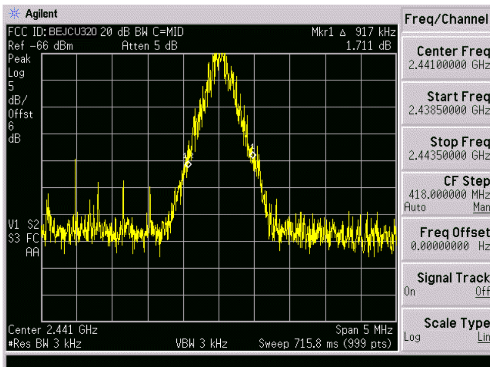
Plot A-2. 20dB Bandwidth Plot – Ch. 45
