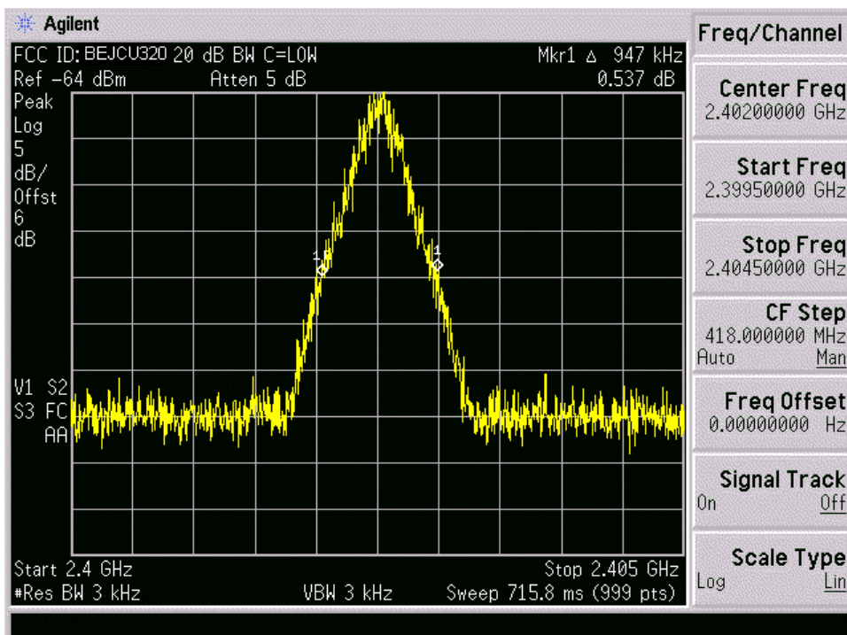
Plot A-1. 20dB Bandwidth Plot – Ch. 01
