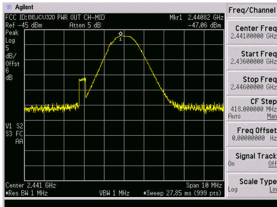
Plot A-5. Max. Peak Output Power Plot – Ch. 45
