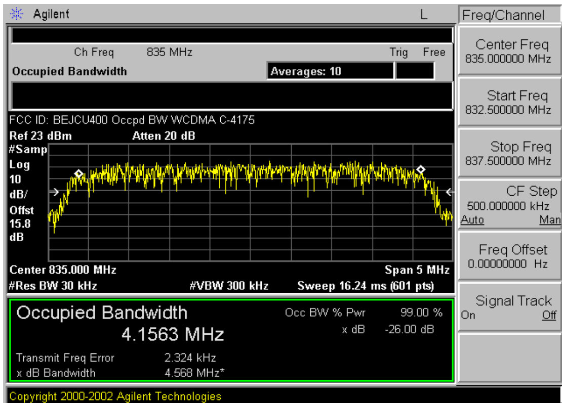
Plot A-7. Occupied Bandwidth Plot (Cellular WCDMA Mode – Ch. 4175)
