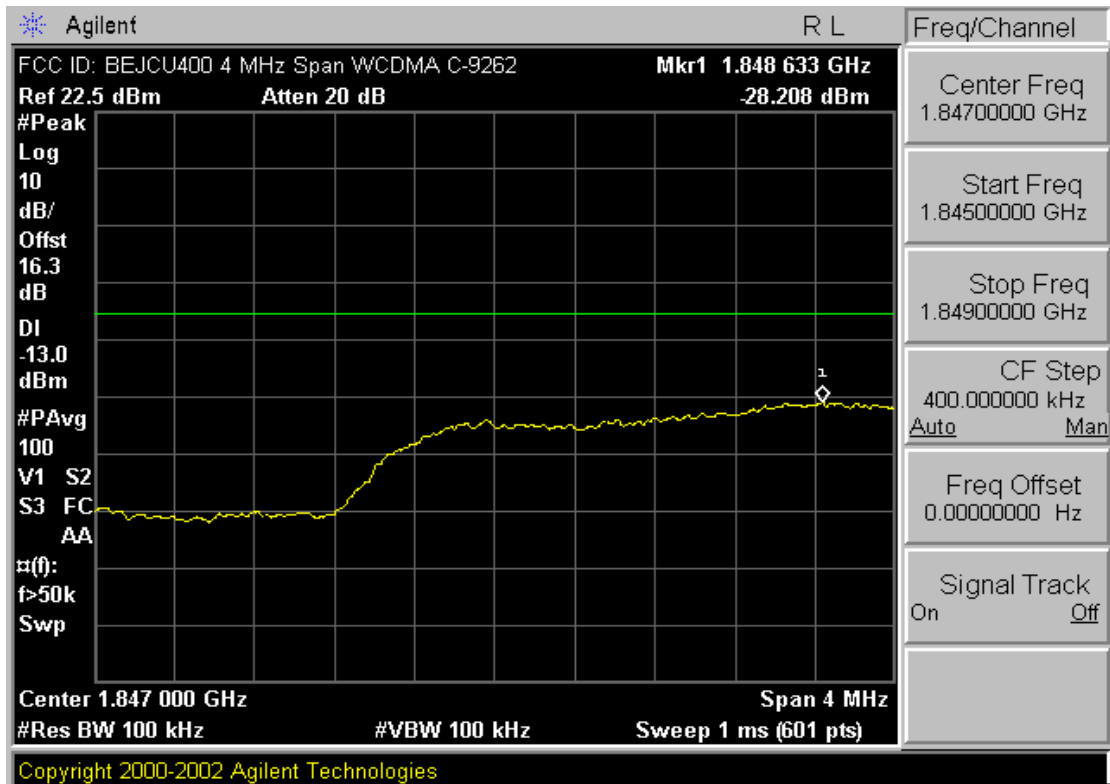
Plot A-16. 4MHz Span Plot (PCS WCDMA Mode – Ch. 9262)
