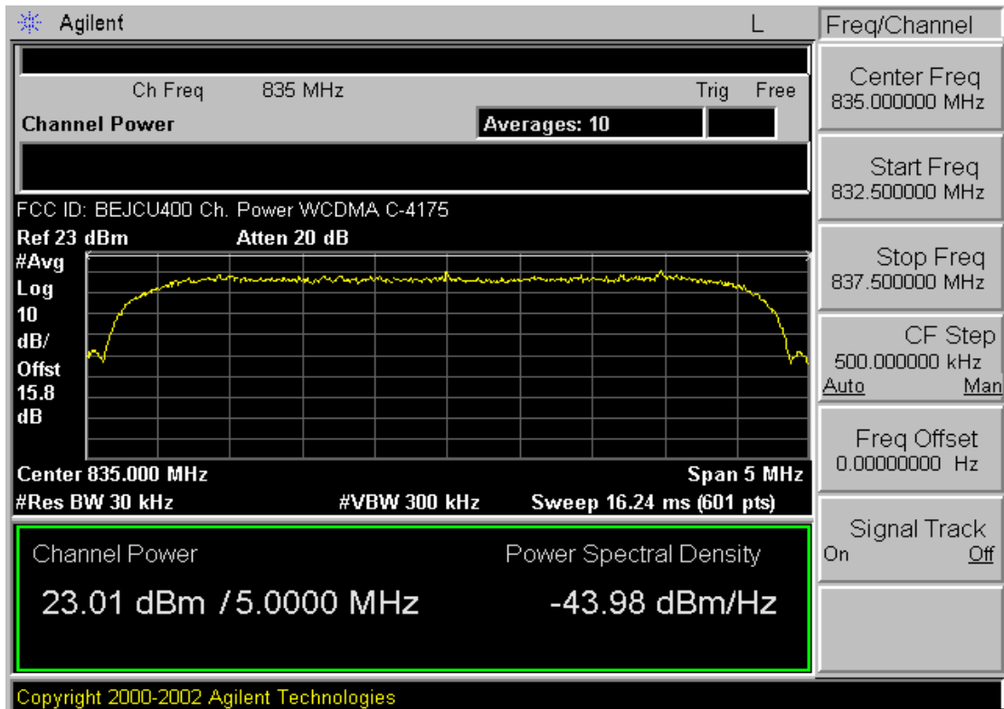
Plot A-8. Channel Power Plot (Cellular WCDMA Mode – Ch. 4175)
