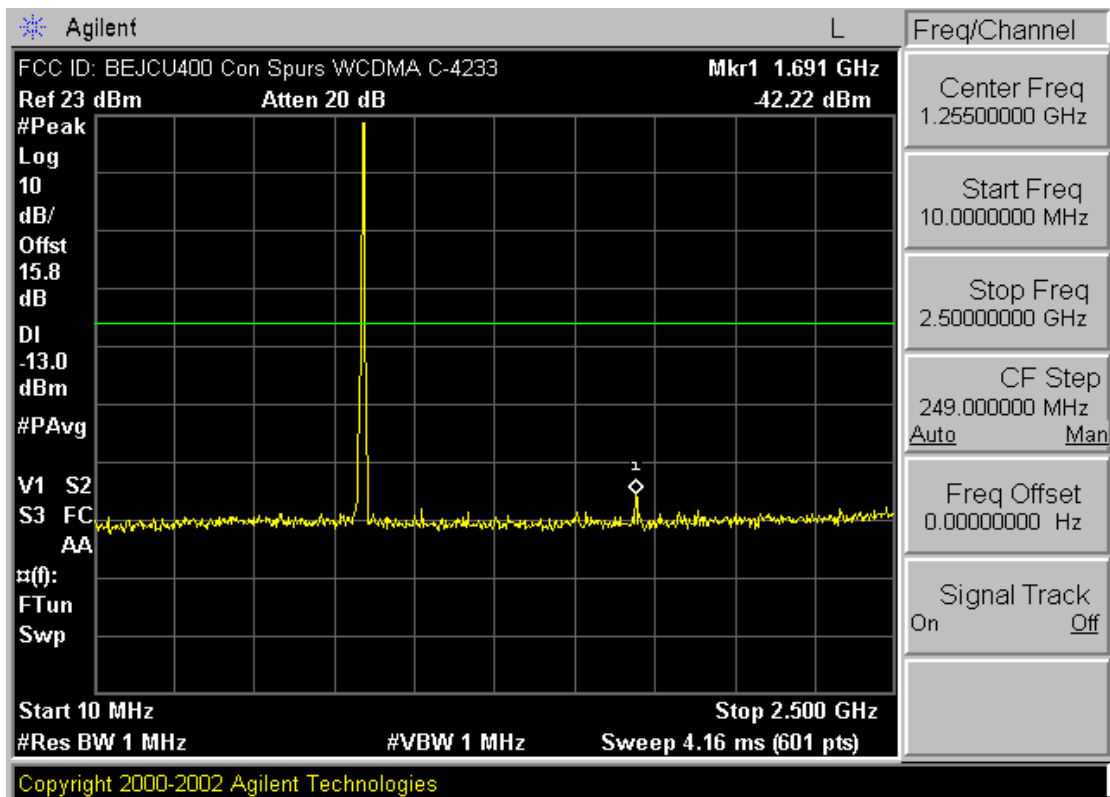
Plot A-9. Conducted Spurious Plot (Cellular WCDMA Mode – Ch. 4233)
