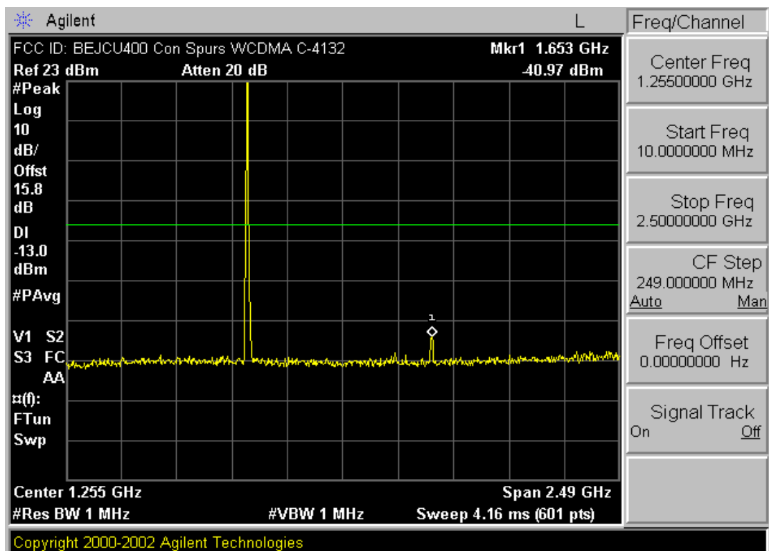
Plot A-1. Conducted Spurious Plot (Cellular WCDMA Mode – Ch. 4132)
