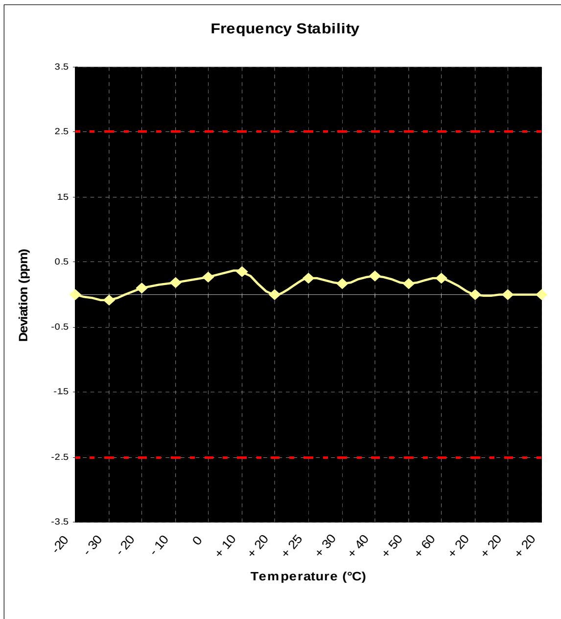
Figure 6-2. Frequency Stability Graph (Cellular WCDMA Mode – Ch. 4175)
