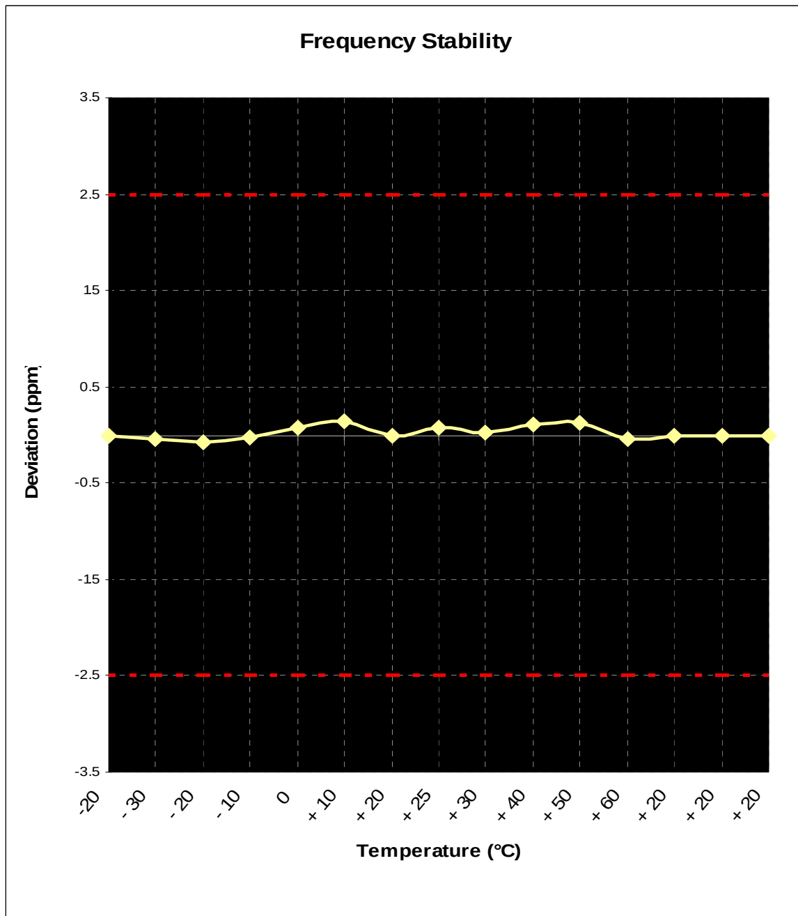
Figure 6-3. Frequency Stability Graph (PCS WCDMA Mode – Ch. 9400)
