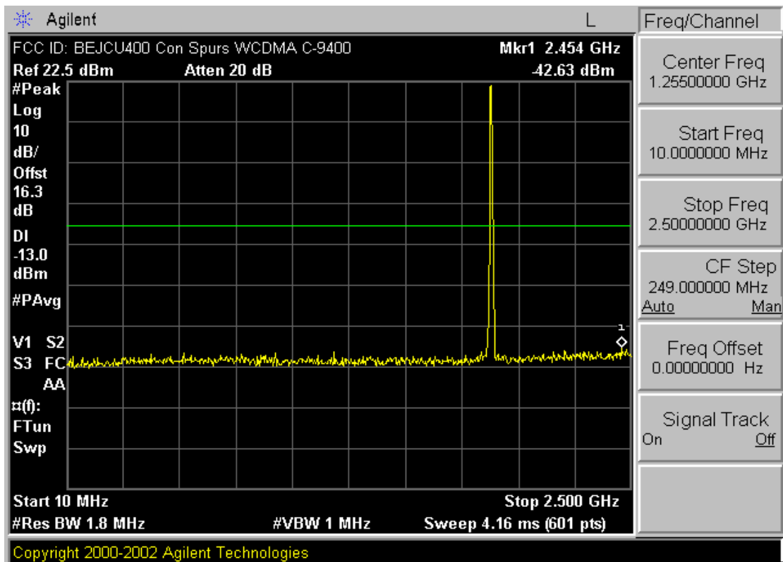
Plot A-17. Conducted Spurious Plot (PCS WCDMA Mode – Ch. 9400)
