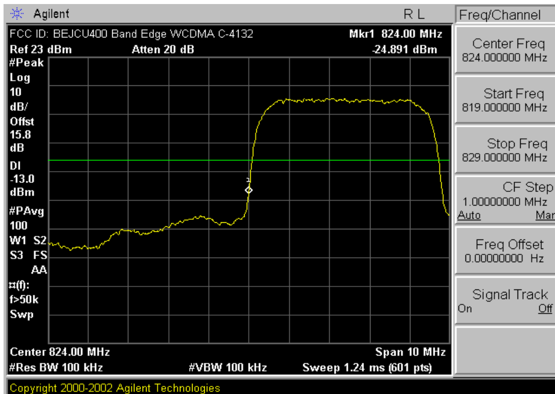
Plot A-3. Band Edge Plot (Cellular WCDMA Mode – Ch. 4132)
