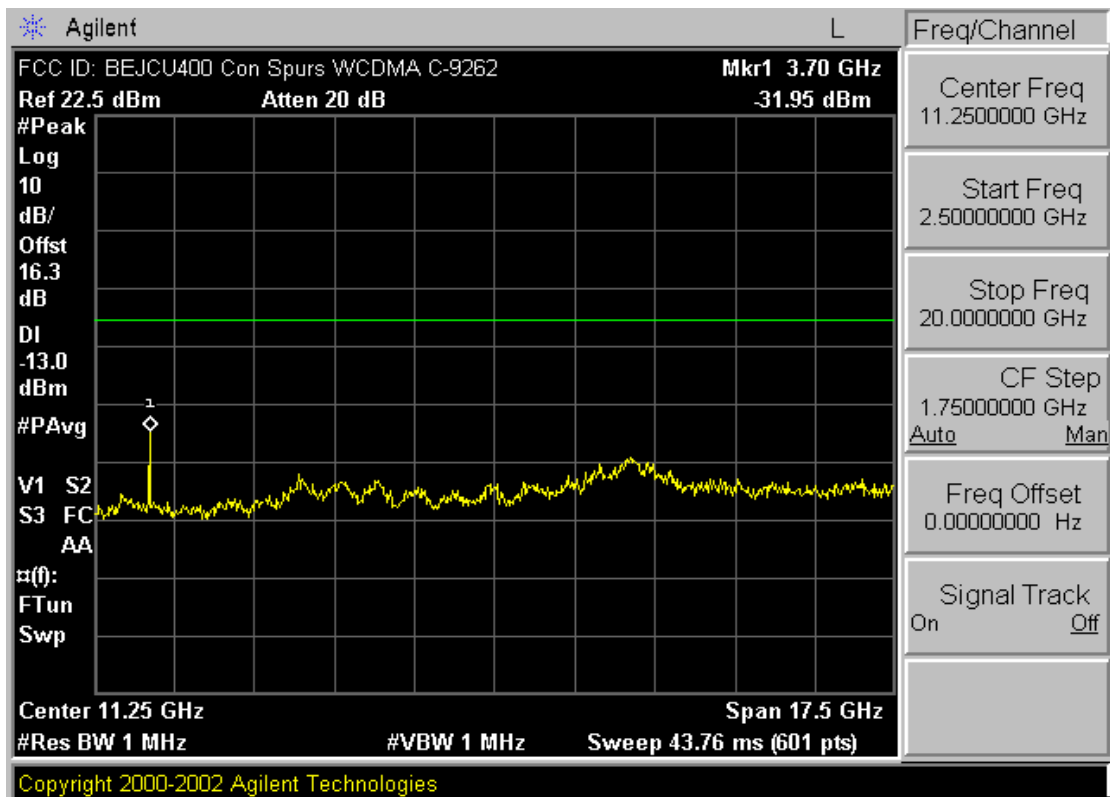
Plot A-14. Conducted Spurious Plot (PCS WCDMA Mode – Ch. 9262)
