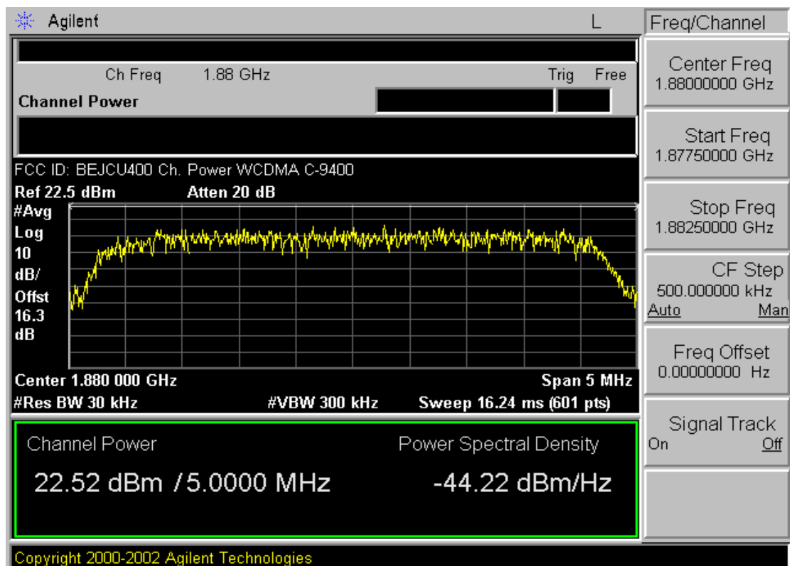
Plot A-20. Channel Power Plot (PCS WCDMA Mode – Ch. 9400)
