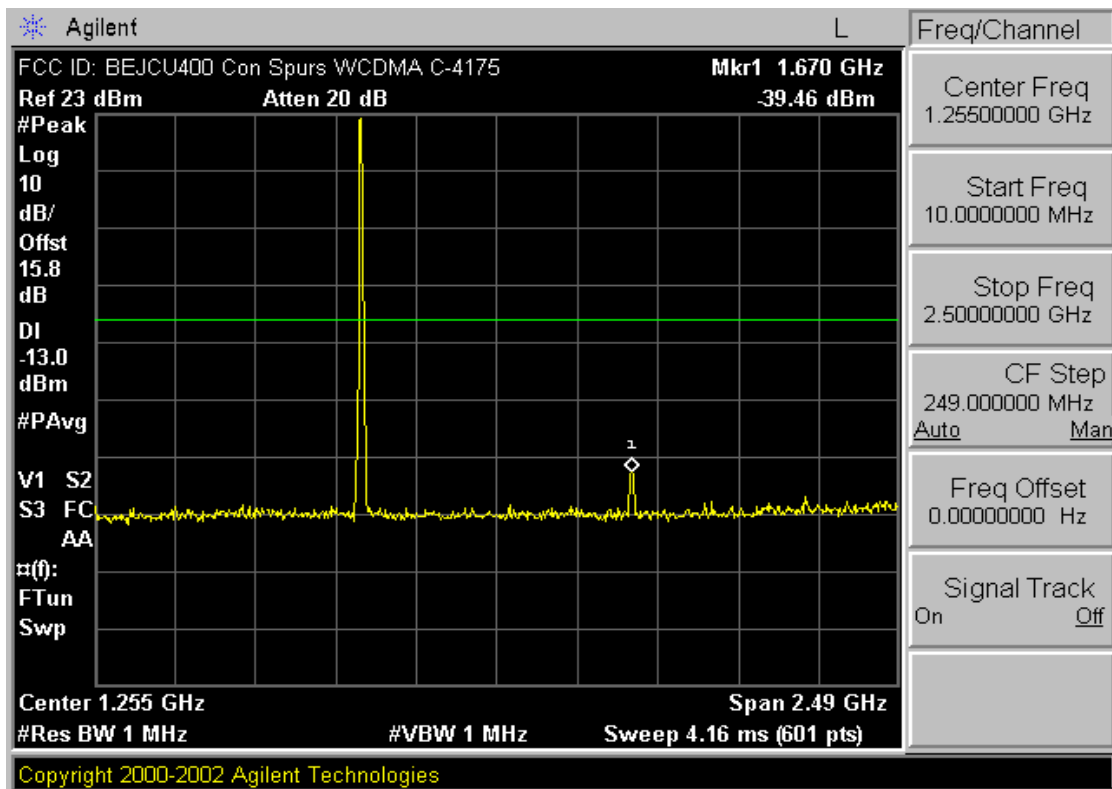
Plot A-5. Conducted Spurious Plot (Cellular WCDMA Mode – Ch. 4175)
