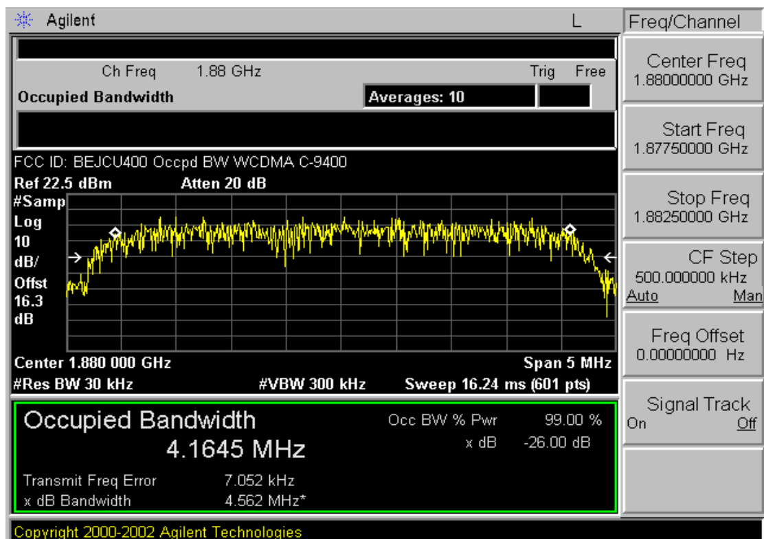
Plot A-19. Occupied Bandwidth Plot (PCS WCDMA Mode – Ch. 9400)
