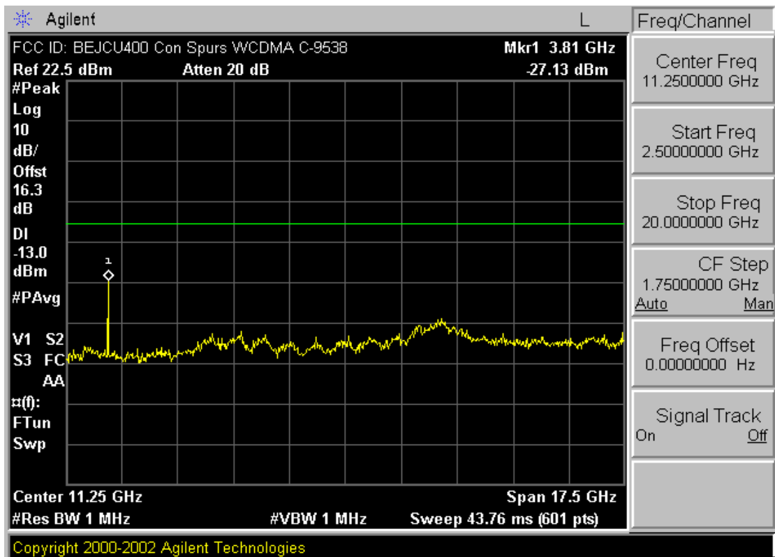
Plot A-22. Conducted Spurious Plot (PCS WCDMA Mode – Ch. 9538)
