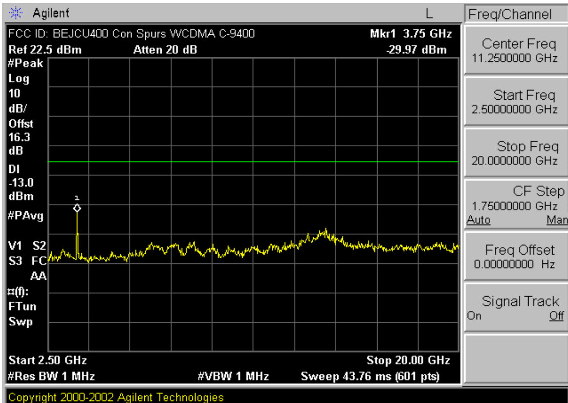
Plot A-18. Conducted Spurious Plot (PCS WCDMA Mode – Ch. 9400)
