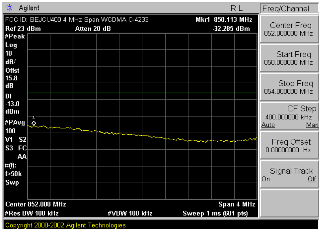
Plot A-12. 4MHz Span Plot (Cellular WCDMA Mode – Ch. 4233)
