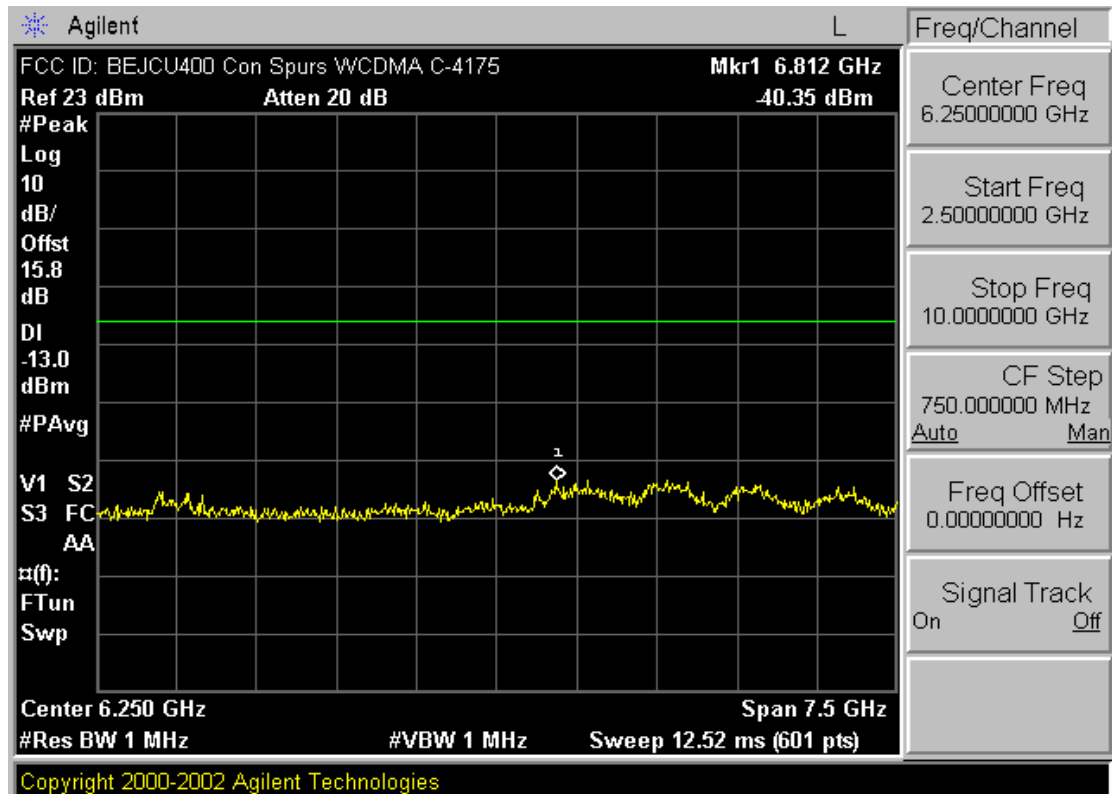
Plot A-6. Conducted Spurious Plot (Cellular WCDMA Mode – Ch. 4175)
