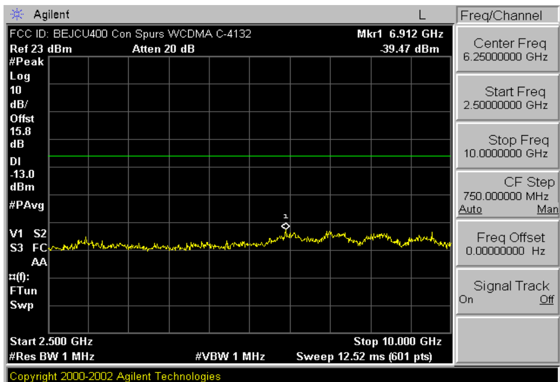
Plot A-2. Conducted Spurious Plot (Cellular WCDMA Mode – Ch. 4132)
