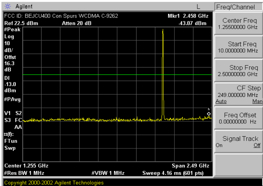
Plot A-13. Conducted Spurious Plot (PCS WCDMA Mode – Ch. 9262)
