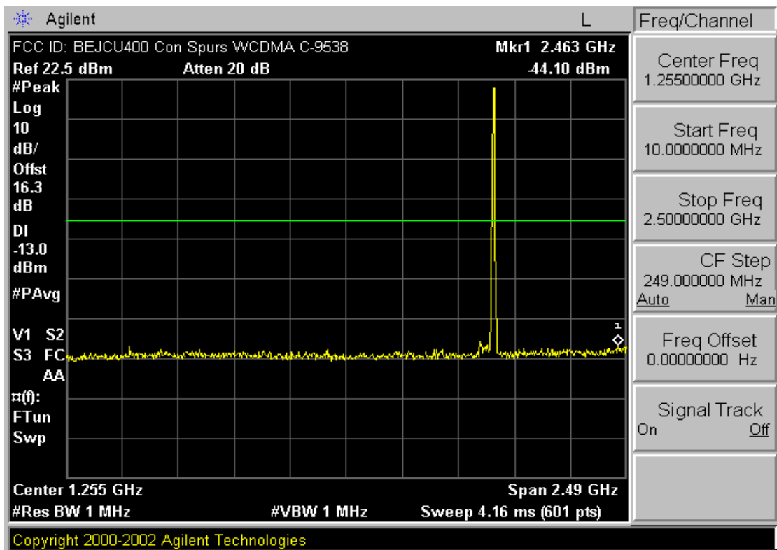
Plot A-21. Conducted Spurious Plot (PCS WCDMA Mode – Ch. 9538)
