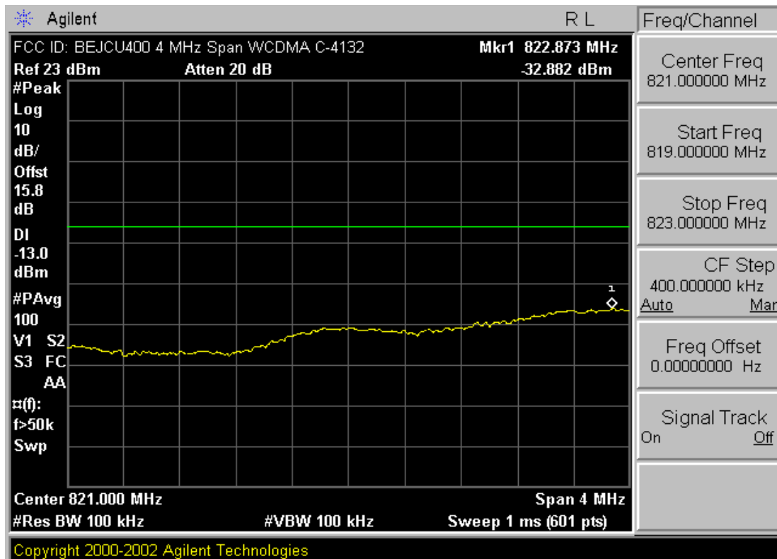
Plot A-4. 4MHz Span Plot (Cellular WCDMA Mode – Ch. 4132)
