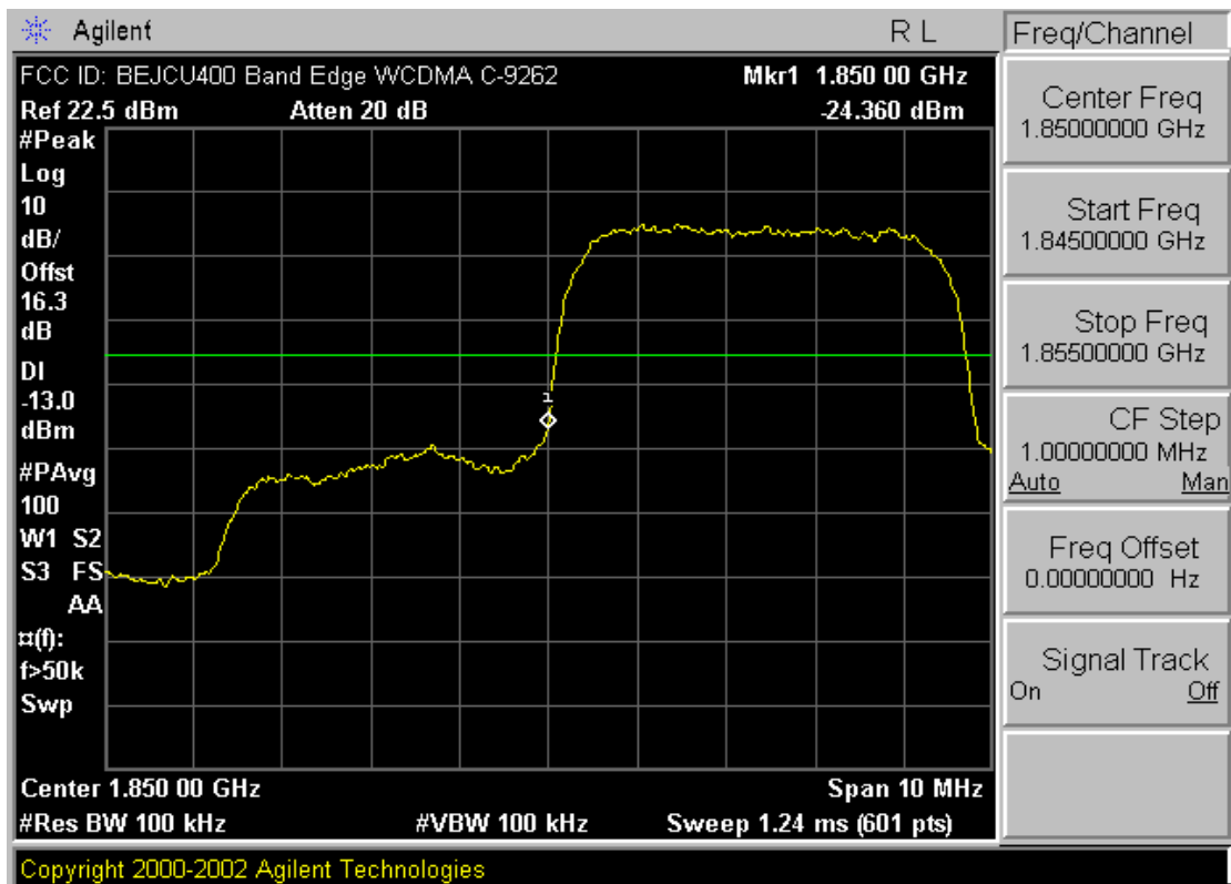
Plot A-15. Band Edge Plot (PCS WCDMA Mode – Ch. 9262)
