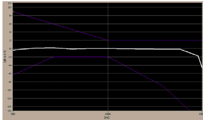
Figure 6-1 Axial Frequency Response
