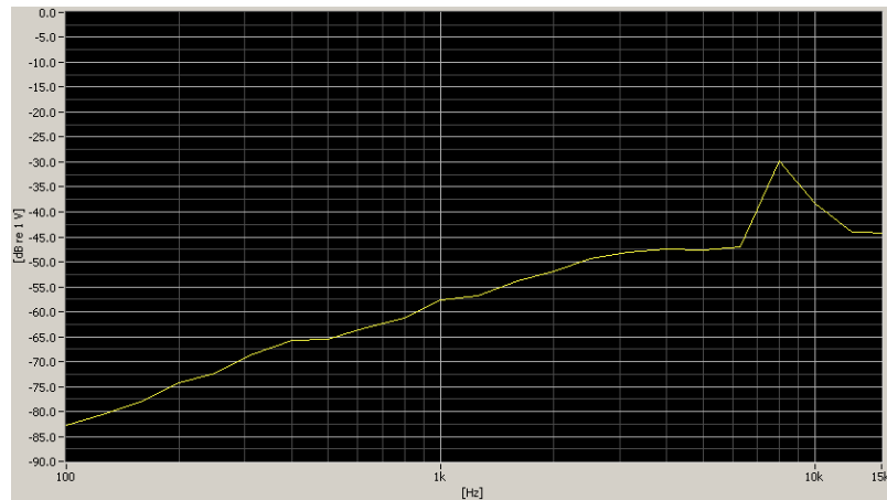
Figure 6-2 Worst-case ABM2 Plot for WD
