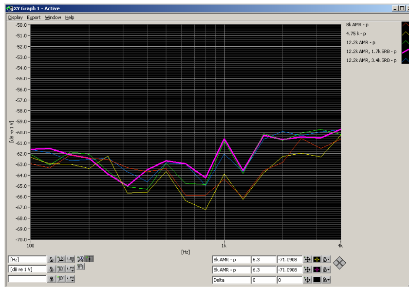
Figure 7-1 WCDMA Audio Band Magnetic Noise
