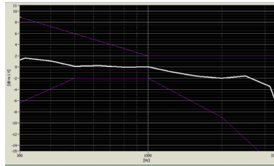
Figure 7-1 Axial Frequency Response
