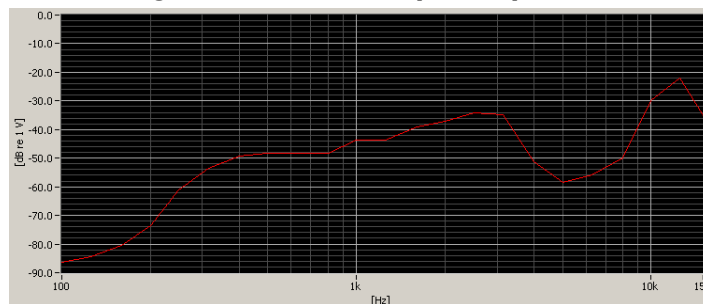
Figure 7-2 Worst-case ABM2 Plot for WD
