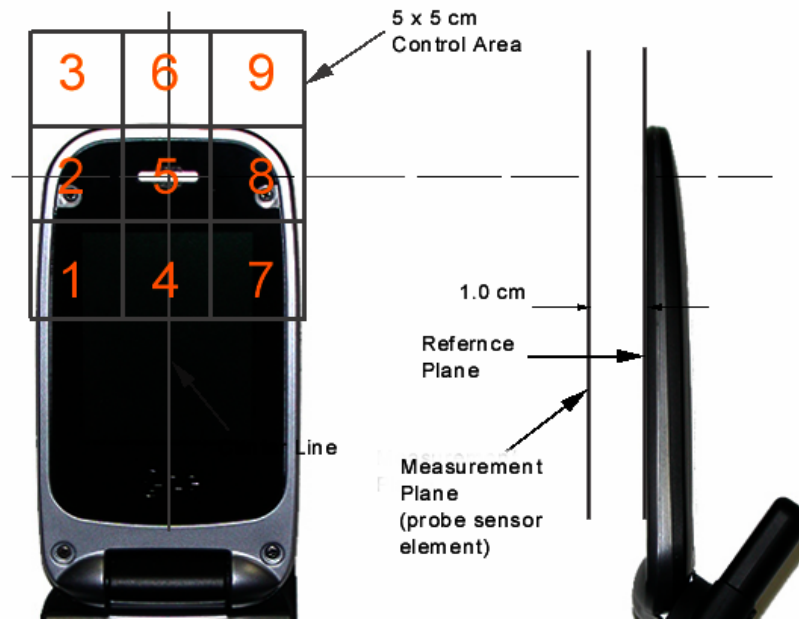
Figure 7 5x5 Scan grid above WD
