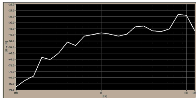
Figure 7-2 Worst-case ABM2 Plot for WD
