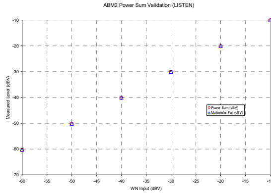
Figure 5-10 ABM2 Power Sum Validation
