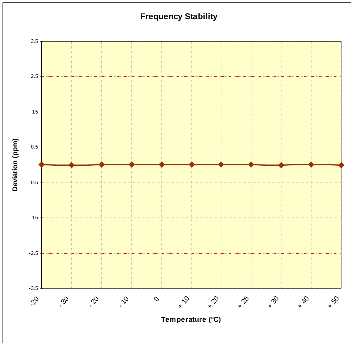
Plot 6-3. Frequency Stability Graph (PCS GSM Mode – Ch. 661)
