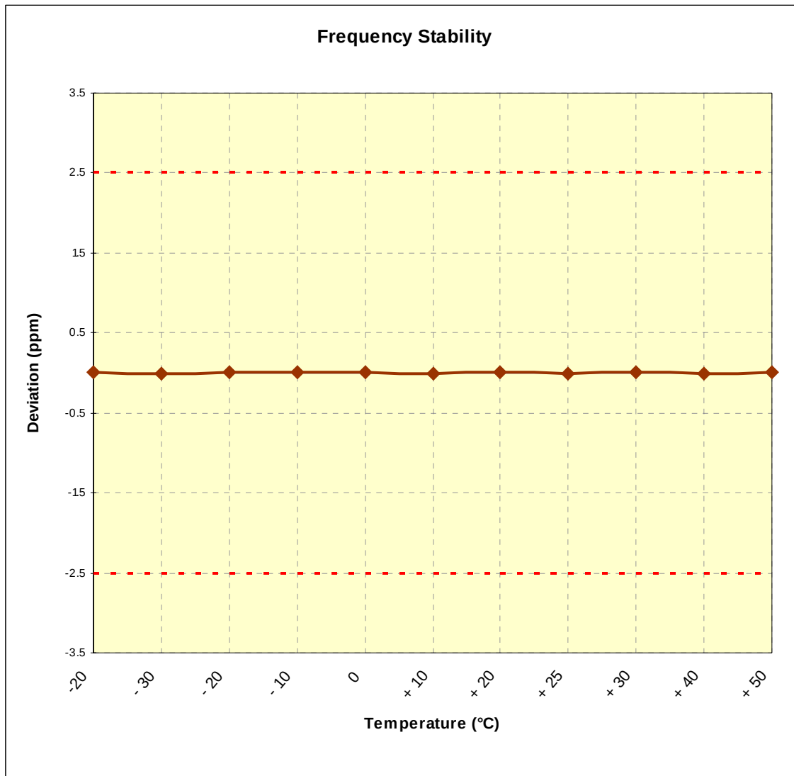
Plot 6-4. Frequency Stability Graph (PCS WCDMA Mode – Ch. 9400)
