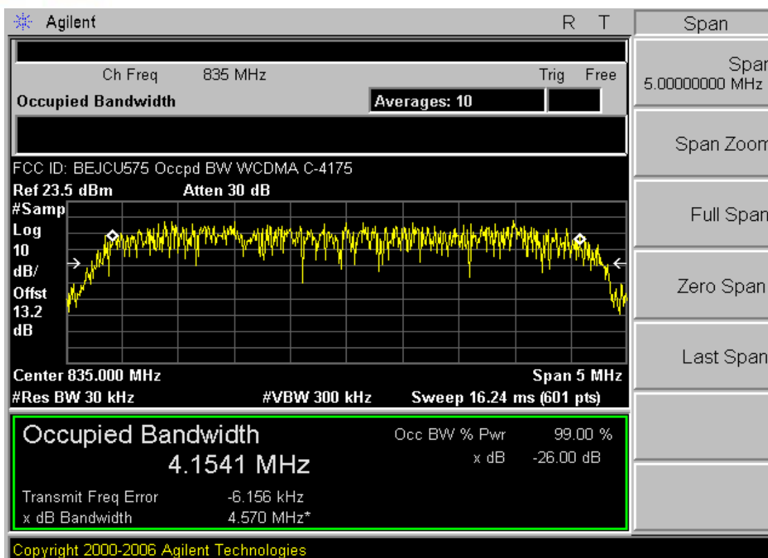
Plot 7-27. Occupied Bandwidth Plot (Cellular WCDMA Mode – Ch. 4175)
