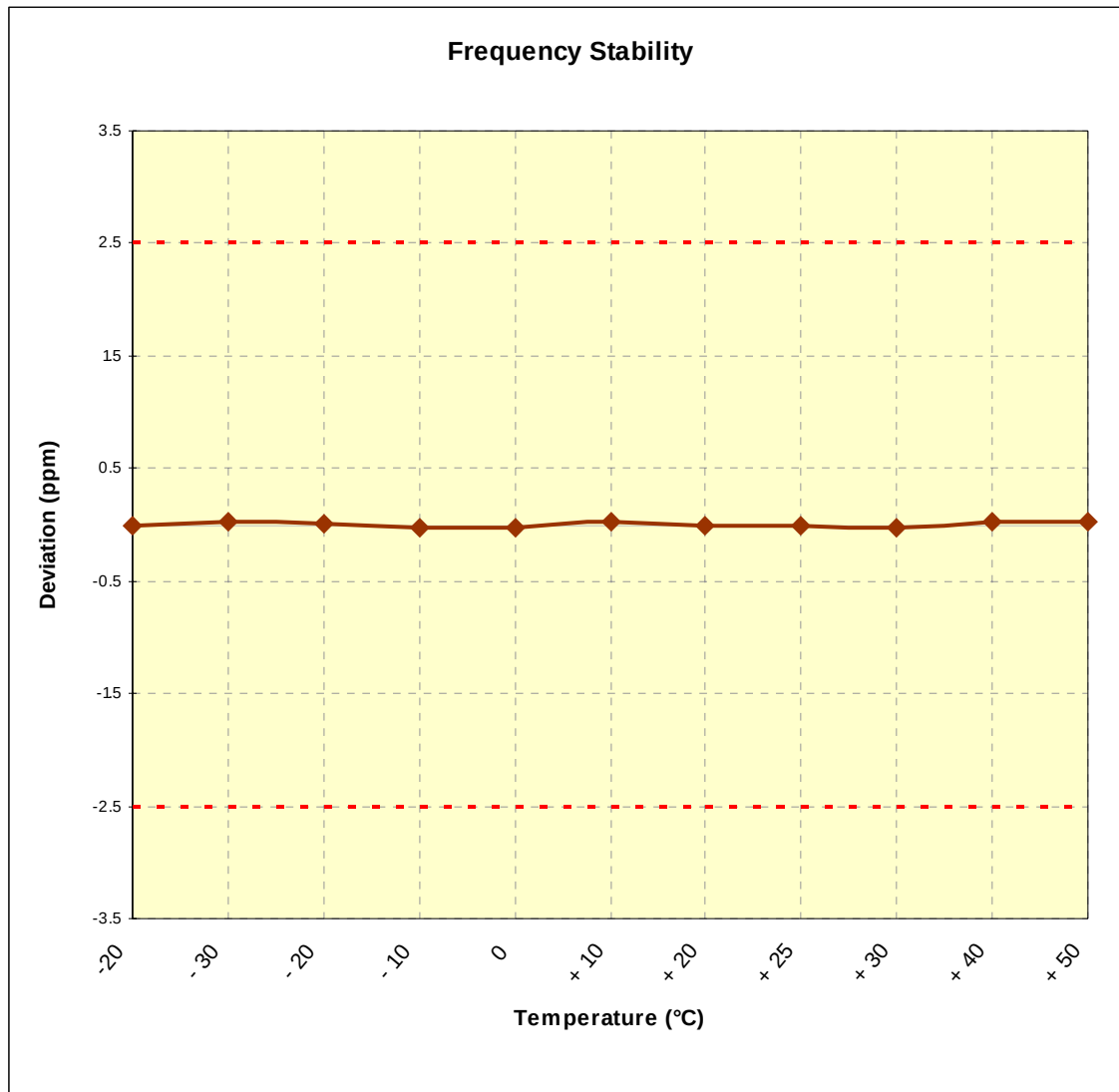
Plot 6-2. Frequency Stability Graph (Cellular WCDMA Mode – Ch. 4175)
