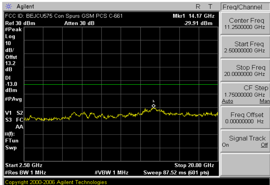
Plot 7-15. Conducted Spurious Plot (PCS GSM Mode – Ch. 661)
