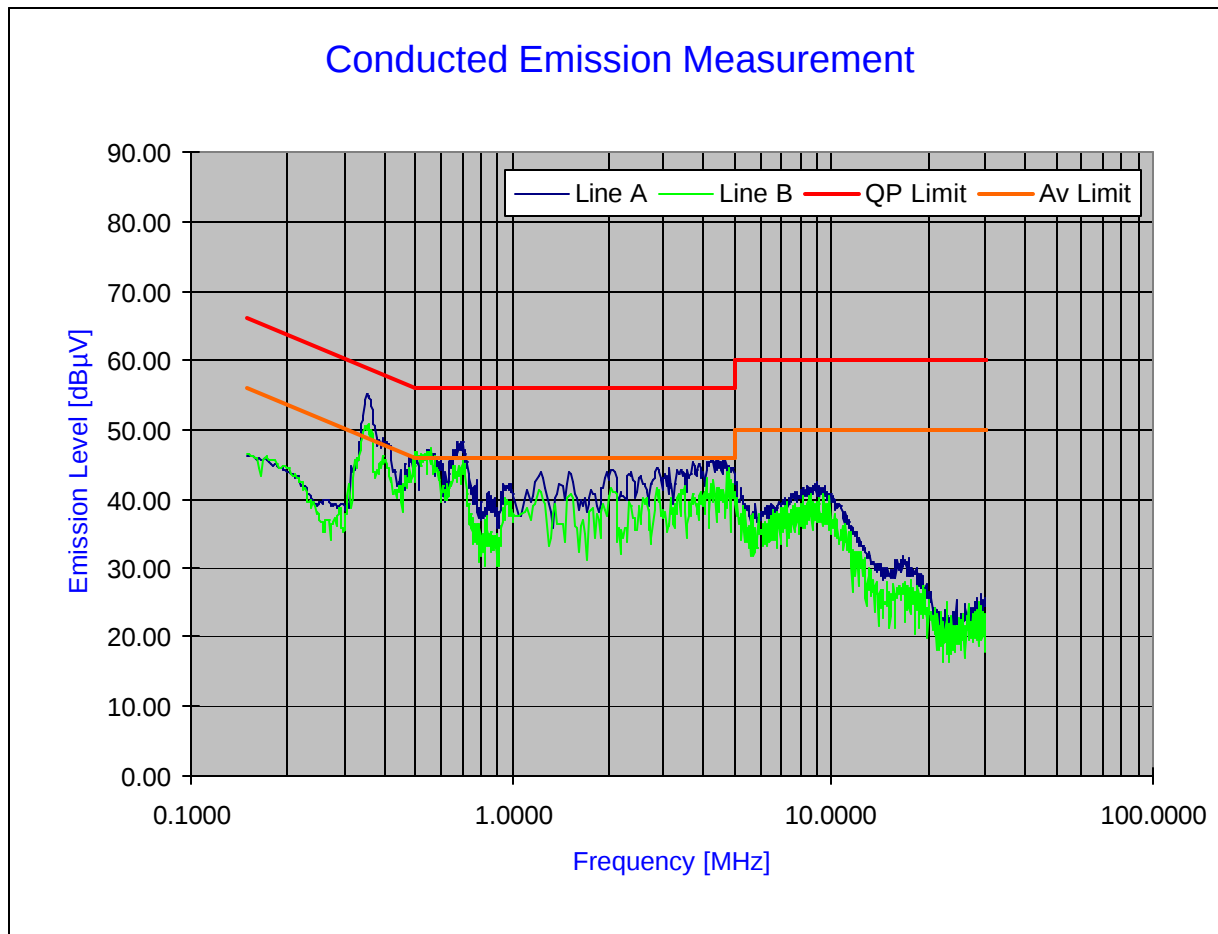
Plot 6-16. Line Conducted Plot with Bluetooth
