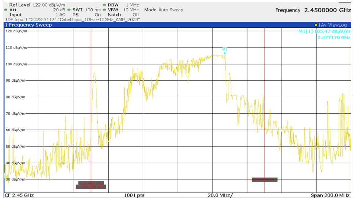
< Fig 7. Frequency Measurements _Voltage (Maximum Frequency Observed: 2.477 GHz) >
