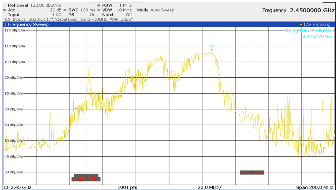
< Fig 9. Frequency Measurements _Load (Maximum Frequency Observed: 2.475 GHz) >
