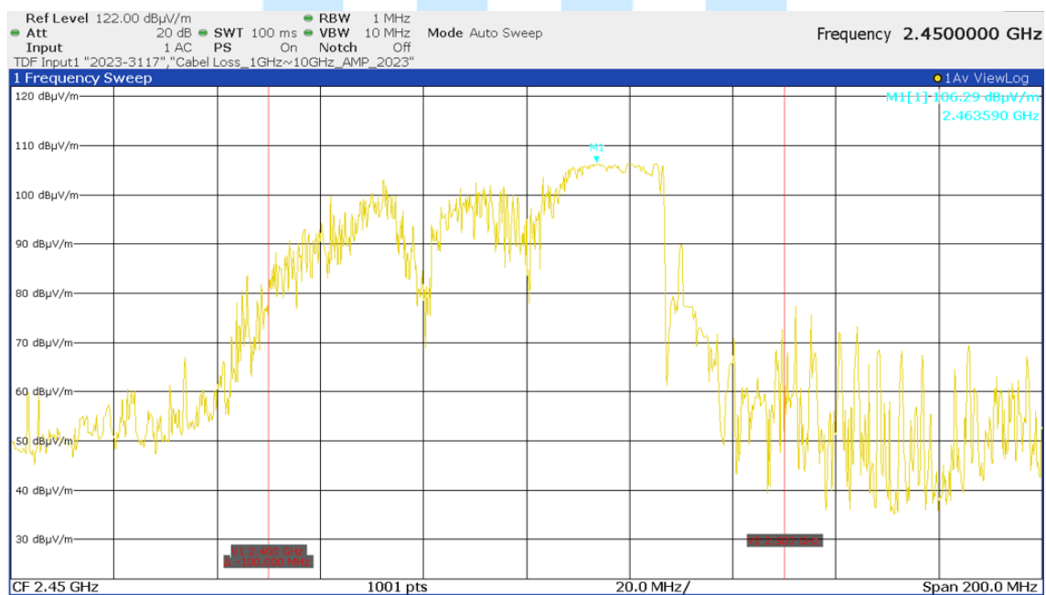
< Fig 10. Frequency Measurements _Load (Minimum Frequency Observed: 2.463 GHz) >
