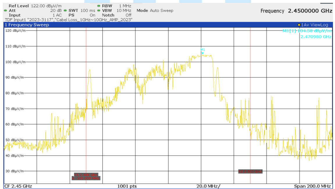
< Fig 8. Frequency Measurements _Voltage (Minimum Frequency Observed: 2.470 GHz) >
