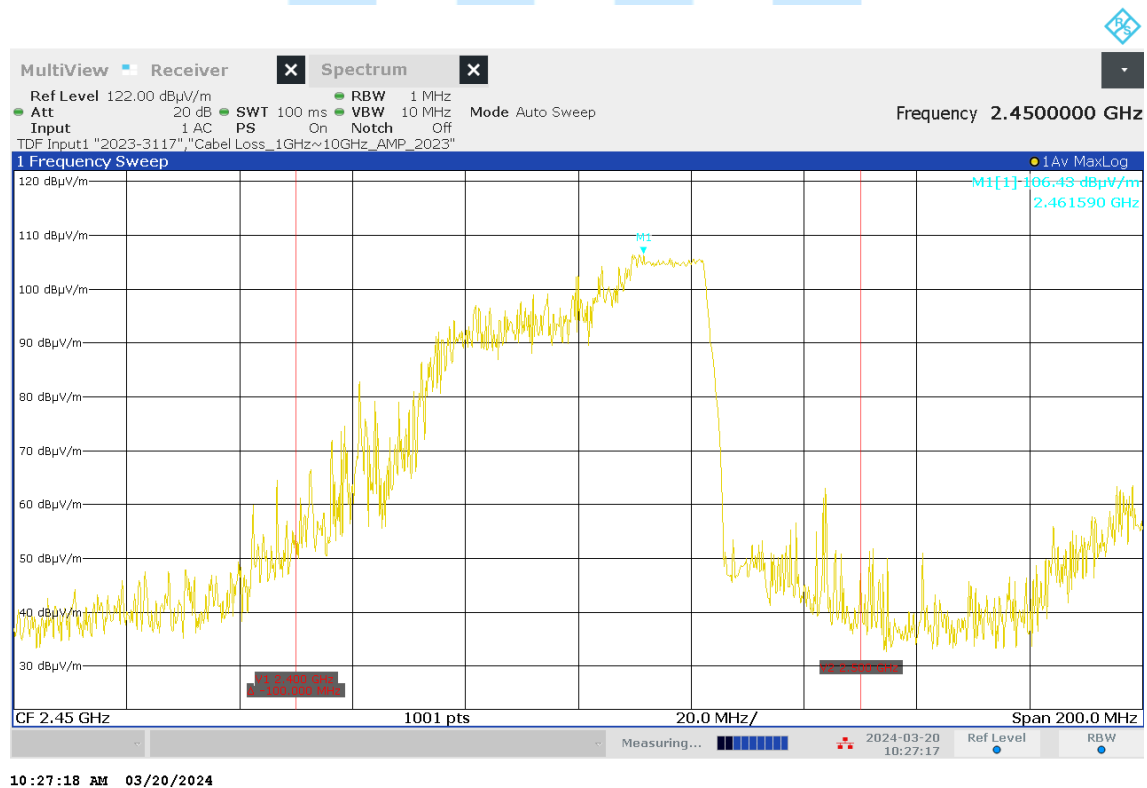
< Fig 10. Frequency Measurements _Load (Minimum Frequency Observed: 2.461 GHz) >
