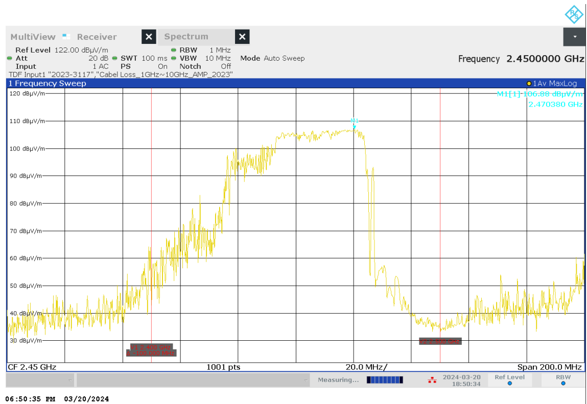
< Fig 7. Frequency Measurements _ Voltage (Maximum Frequency Observed: 2.470 GHz) >
