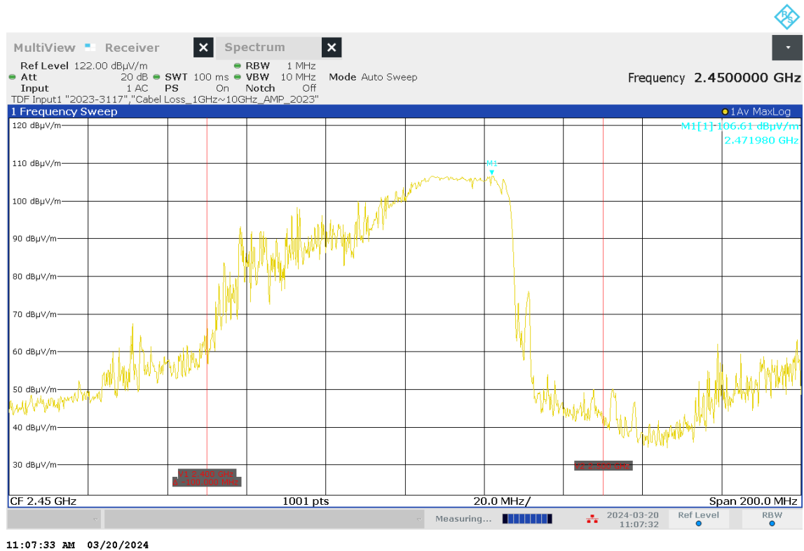
< Fig 9. Frequency Measurements _Load (Maximum Frequency Observed: 2.471 GHz) >
