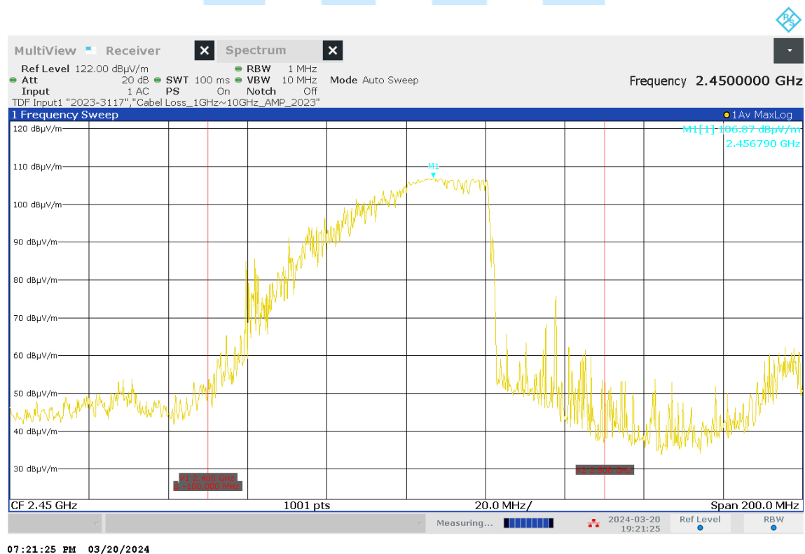
< Fig 8. Frequency Measurements _ Voltage (Minimum Frequency Observed: 2.456 GHz) >
