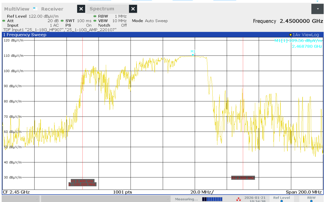
< Fig 10. Frequency Measurements _Load (Minimum Frequency Observed: 2.468 GHz) >
