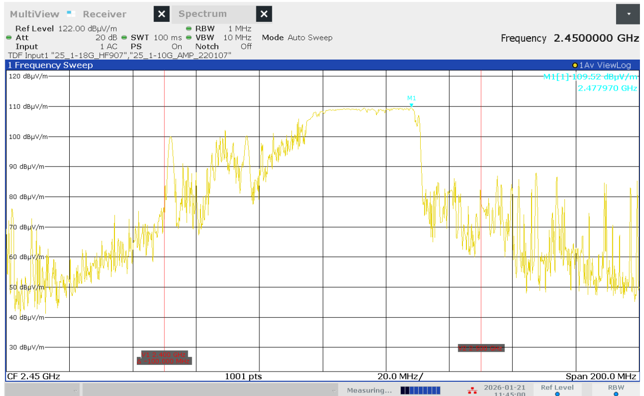
< Fig 7. Frequency Measurements _ Voltage (Maximum Frequency Observed: 2.477 GHz) >
