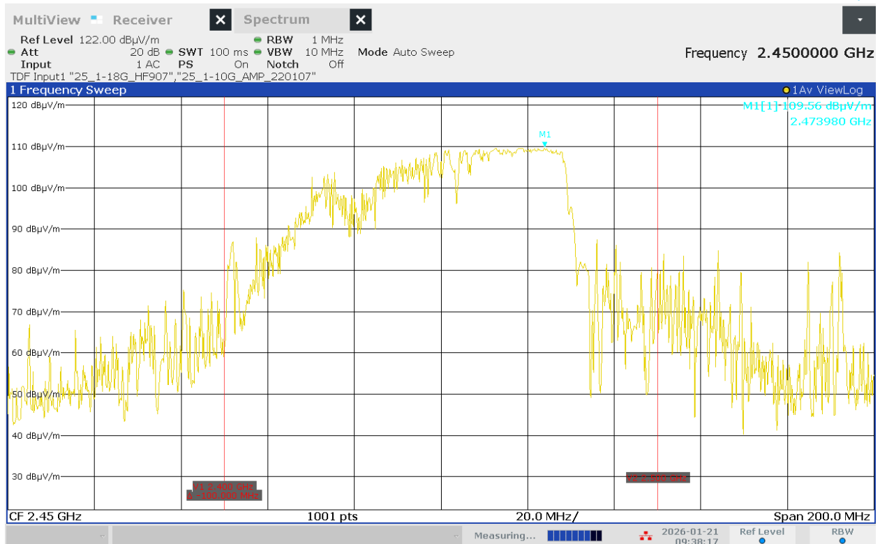
< Fig 9. Frequency Measurements _Load (Maximum Frequency Observed: 2.473 GHz) >
