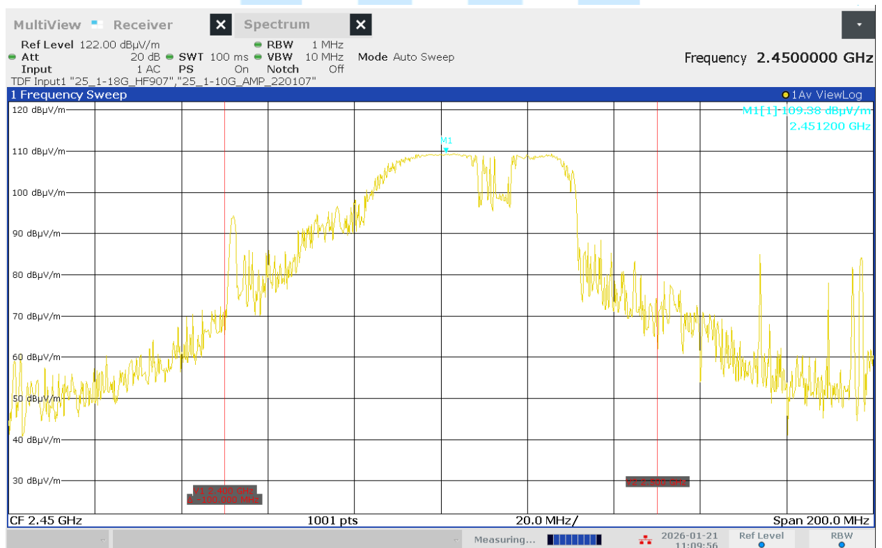
< Fig 8. Frequency Measurements _ Voltage (Minimum Frequency Observed: 2.451 GHz) >
