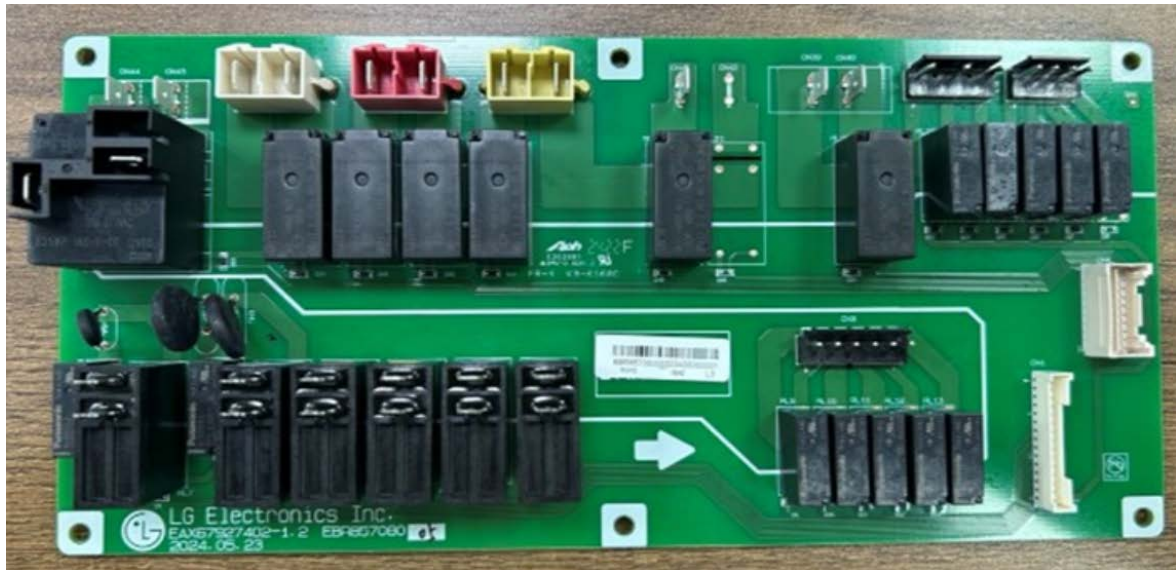
<PCB – Top of Relay board>
