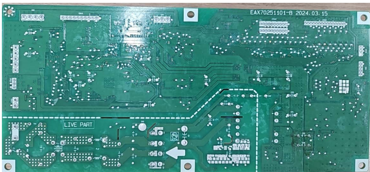
<PCB – Bottom of Main board>
