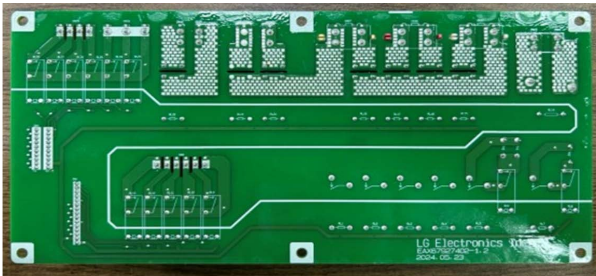
<PCB – Bottom of Relay board>
