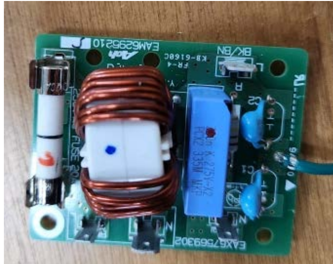
<Top of Noise filter>
