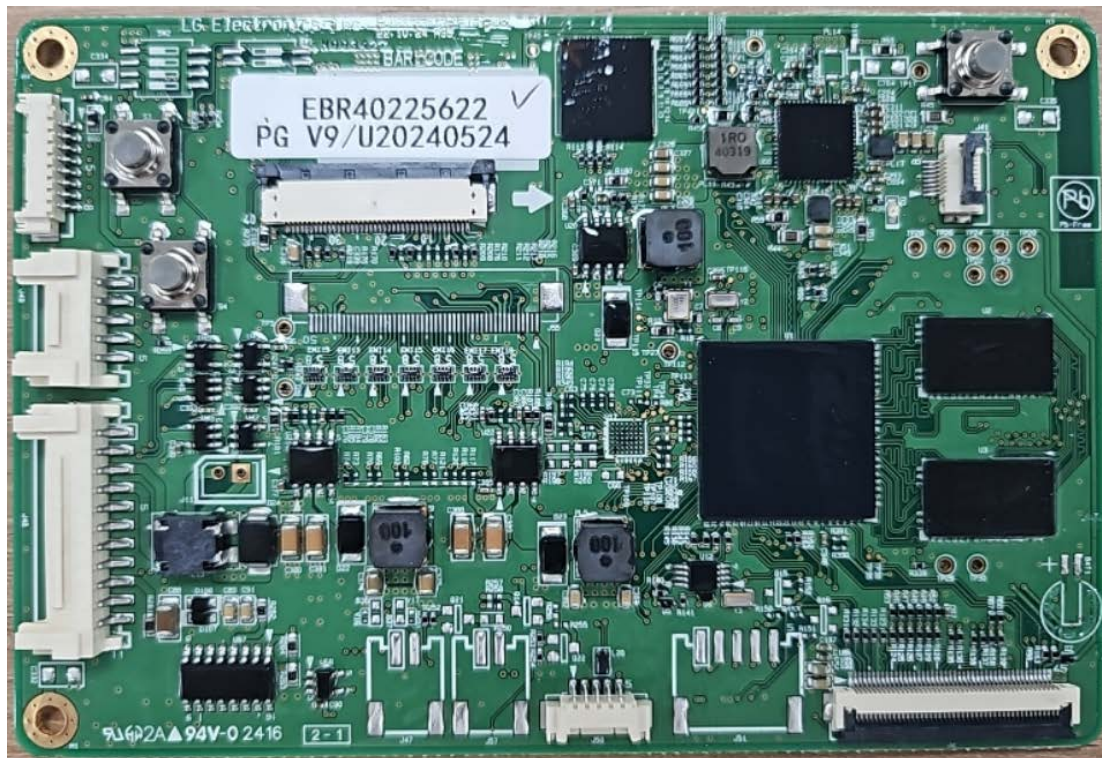
<PCB – Top of Display board>
