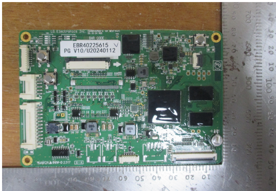
<PCB – Top of Display board>
