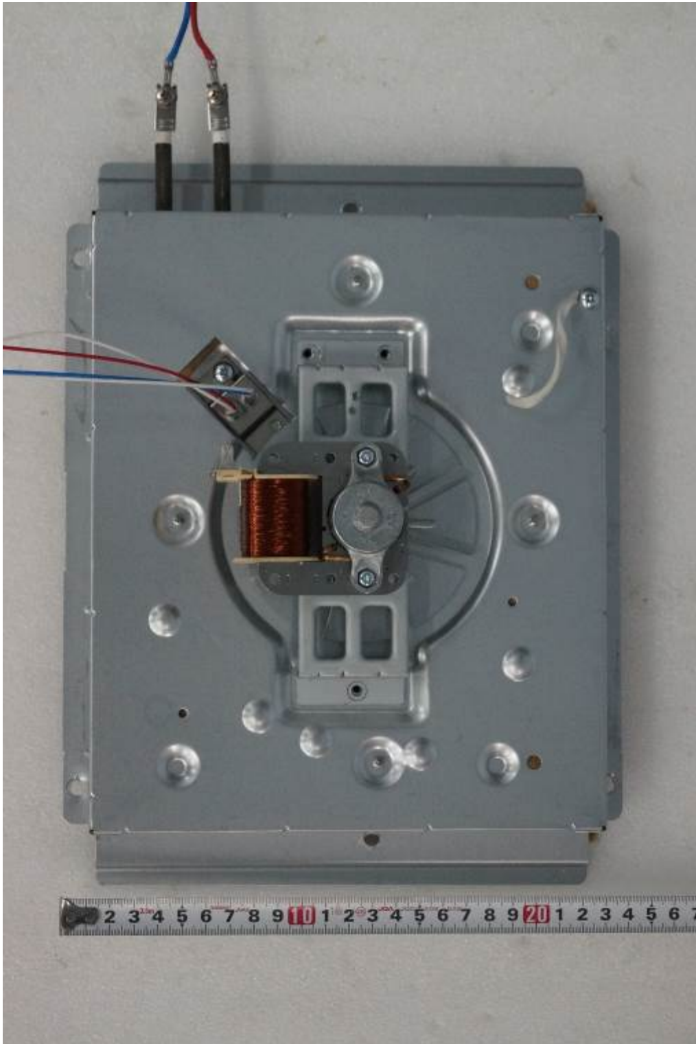
< Machine Section >
