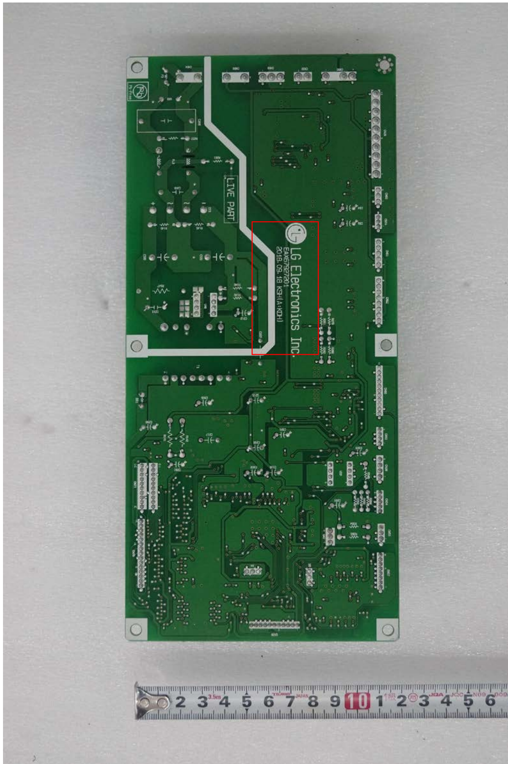
<PCB Section _New>
