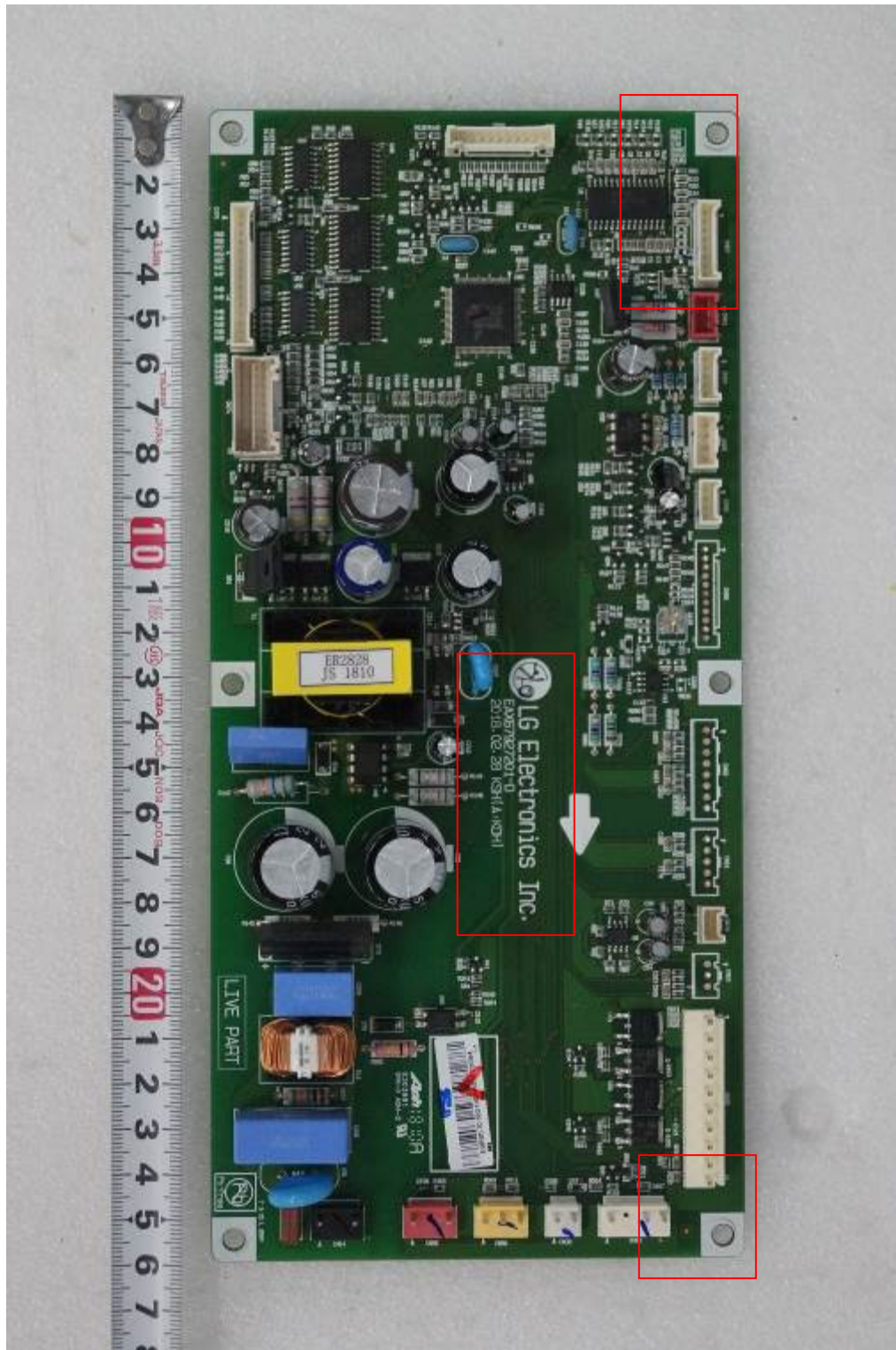
<PCB Section _Original>
