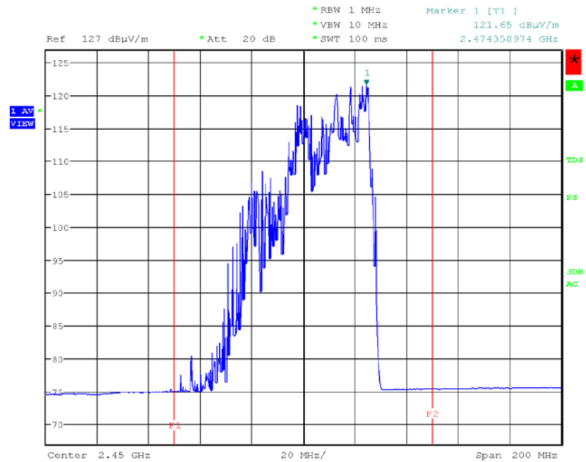
< Fig 7. Frequency Measurements (Maximum Frequency Observed: 2.474 GHz) >
