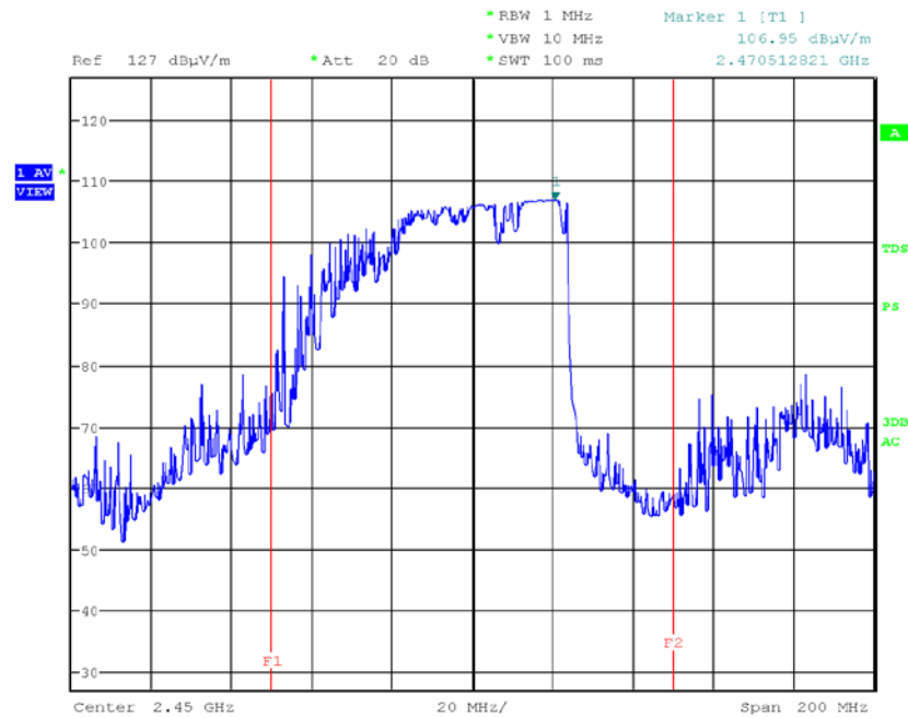
< Fig 7. Frequency Measurements_Load (Maximum Frequency Observed: 2.470 GHz) >
