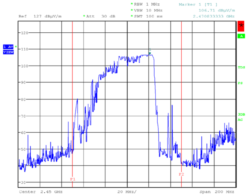
< Fig 9. Frequency Measurements_Voltage (Maximum Frequency Observed: 2.470 GHz) >
