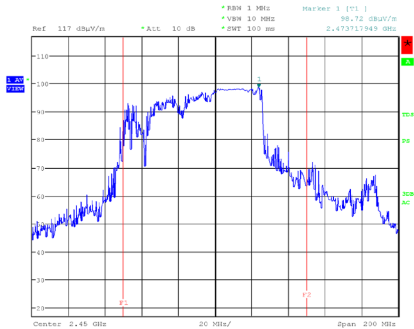
< Fig 9. Frequency Measurements _Load (Maximum Frequency Observed: 2.473 GHz) >
