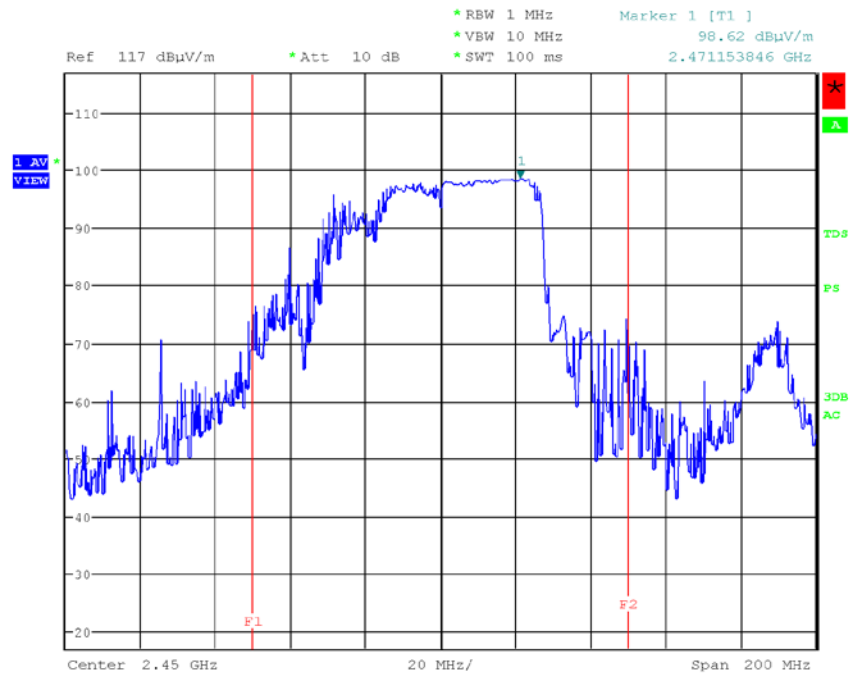
< Fig 7. Frequency Measurements _ Voltage (Maximum Frequency Observed: 2.471 GHz) >
