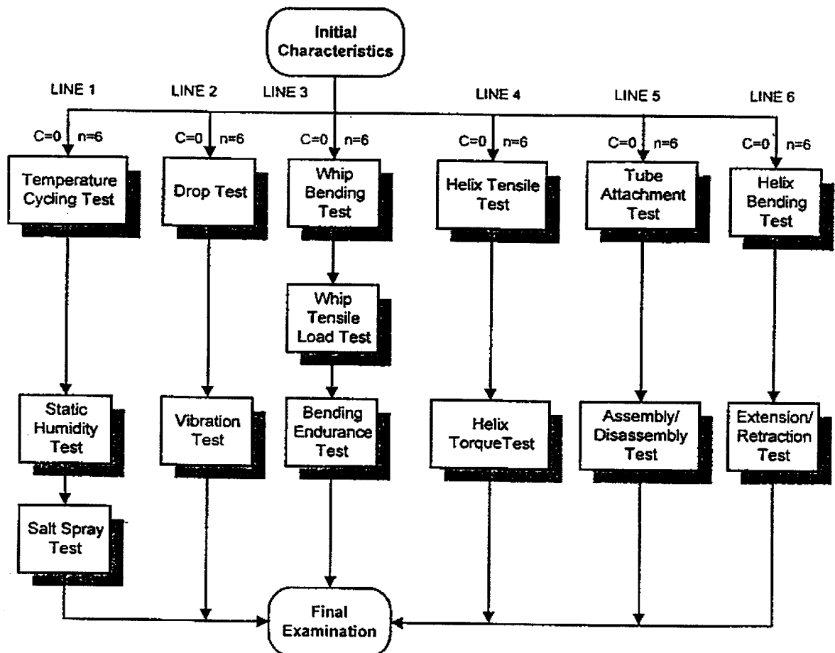
Figure 5. Qualification Flow Chart Allowed amount of failures after every test line c=0 ; Sample size n=6
