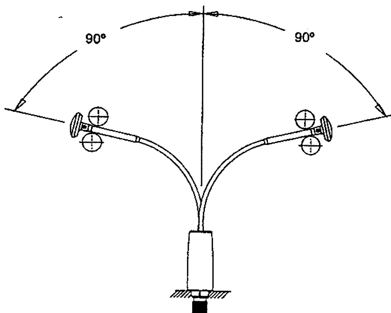
Figure 4. Method for Whip Bending Endurance Testing
